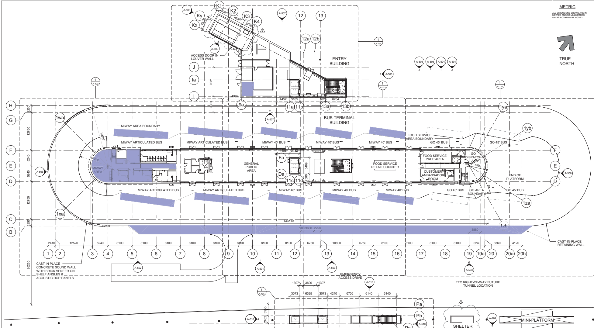
1 OVERALL PLAN 1 : 250
