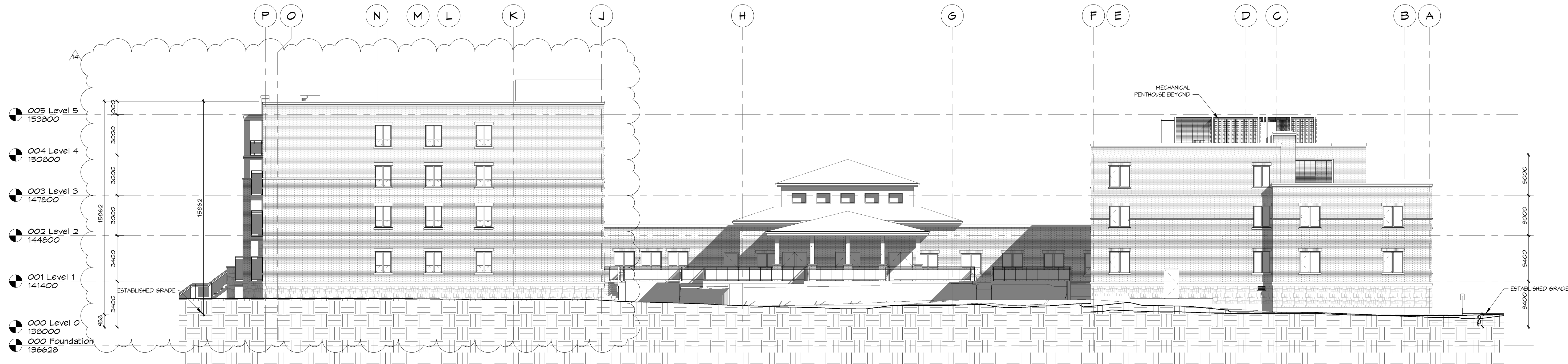
2 West A301 1: 150
