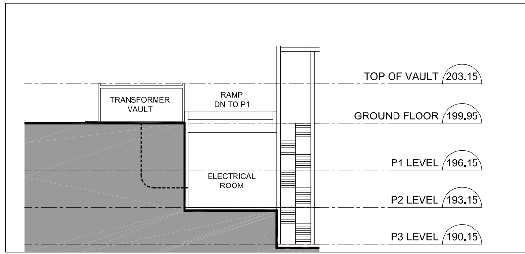
2 TRANSFORMER VAULT & ELECTRICAL ROOM 1:300
