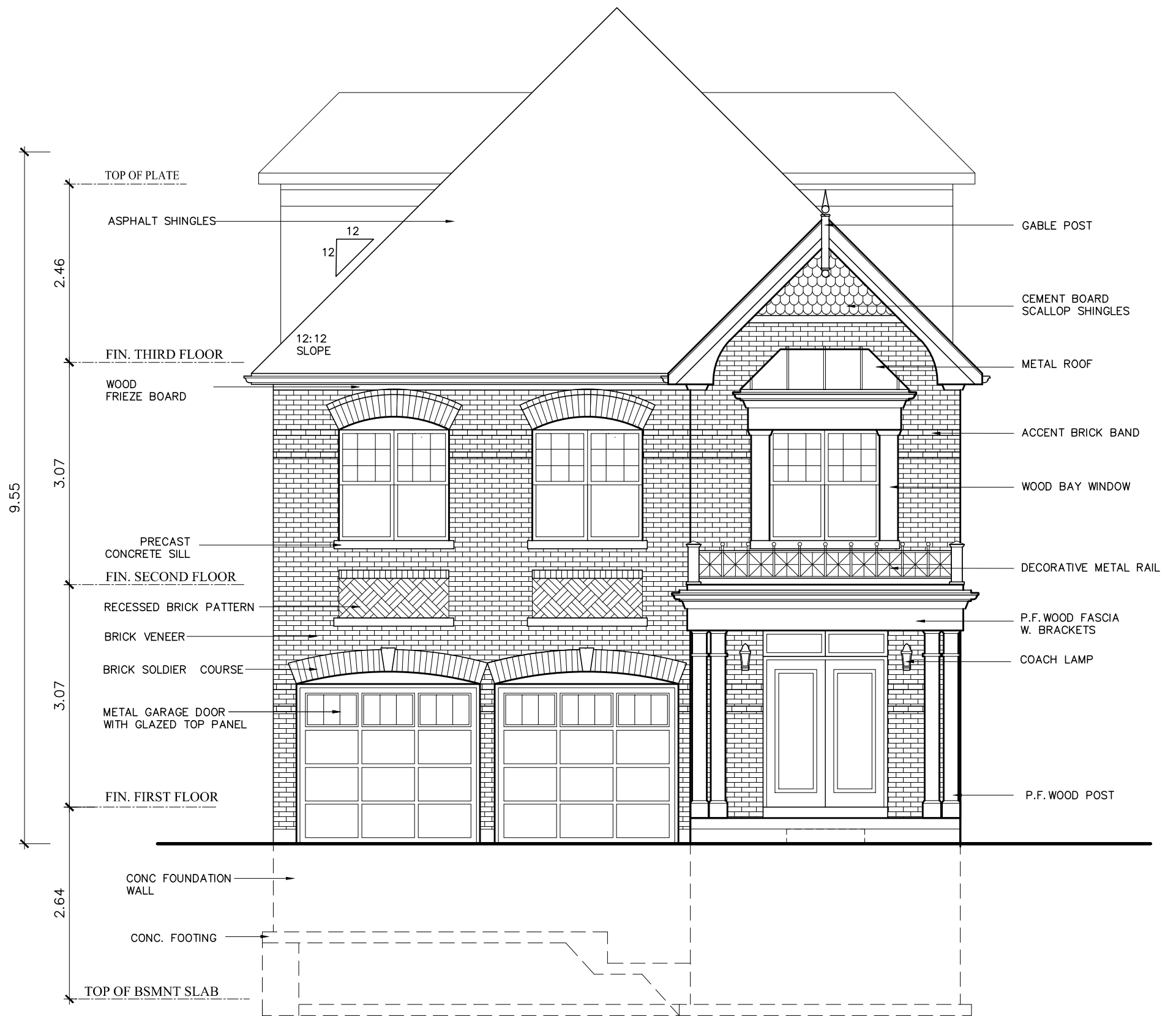
MODEL B FRONT ELEVATION B / LOT 23
