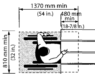
Figure 4.3.7.2 Frontal Approach
