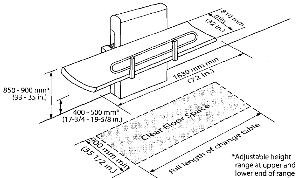
Figure 4.2.7.2 Adult Change Table
