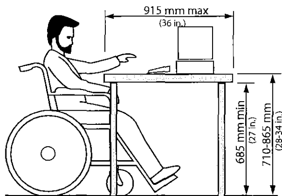
Figure 4.5.6.3 Work Surfaces
