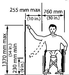
Figure 4.1.1.9 Side Reach
