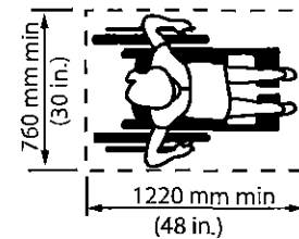
Figure 4.1.1.5 Clear Floor Space for Wheelchair
