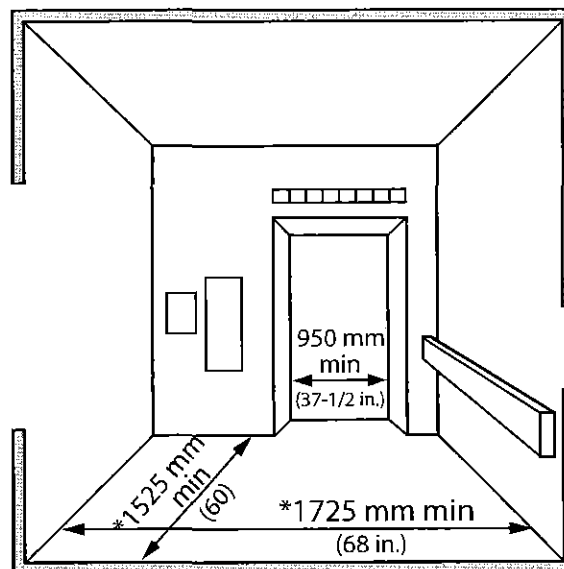
Figure 4.1.14.1 Elevator Cab
