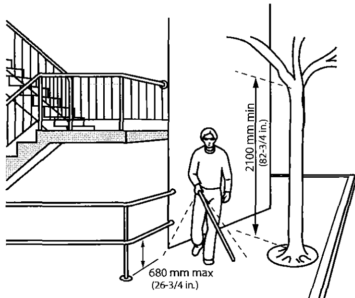
Figure 4.1.3.3 Overhead Obstructions
