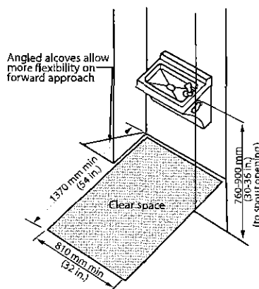
Figure 4.3.1.2 Forward Approach
