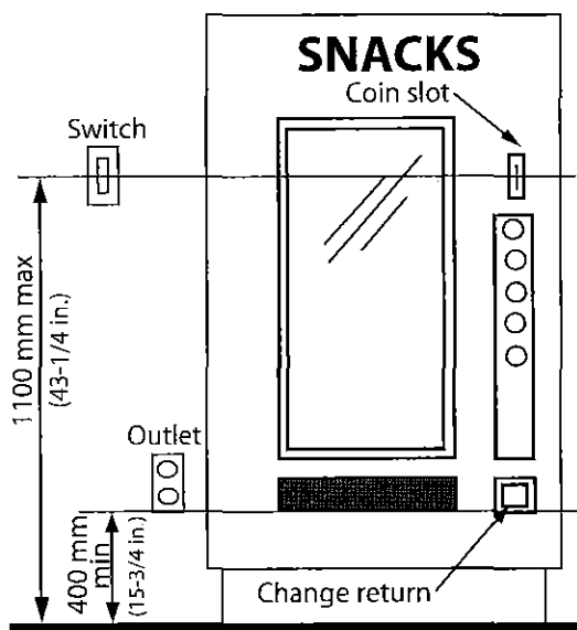
Figure 4.4.3.1 Vending Machine
