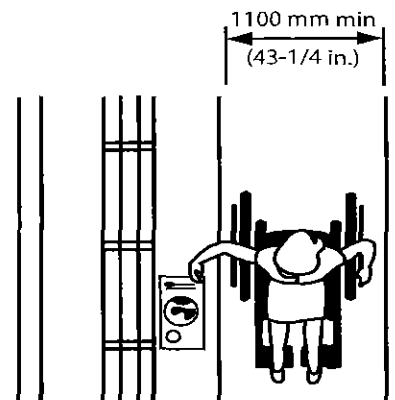
Figure 4.5.4.2 Aisle Width
