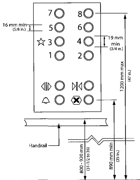
Figure 4.1.14.2 Control Panel
