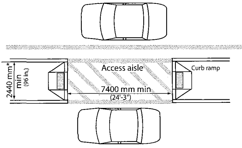
Figure 4.3.13.2 Passenger Loading Zone
