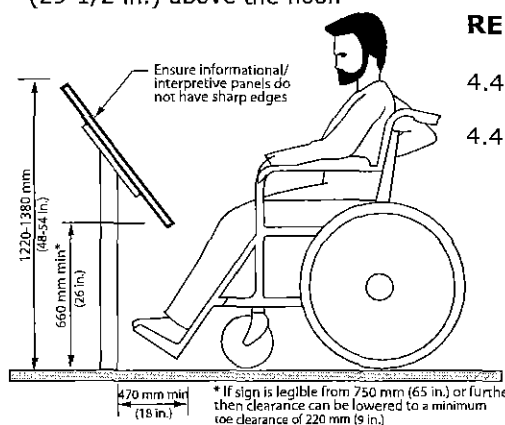
Figure 4.4.10.1 Critical dimensions for information systems and displays
