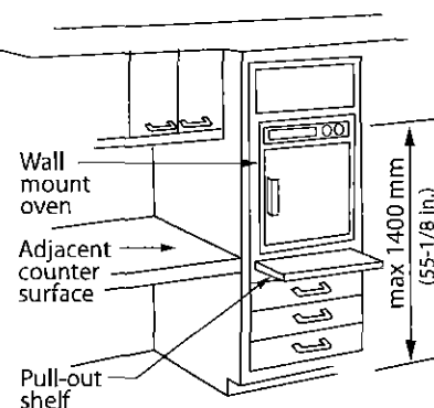
Figure 4.3.18.8 Wall-Mounted Oven
