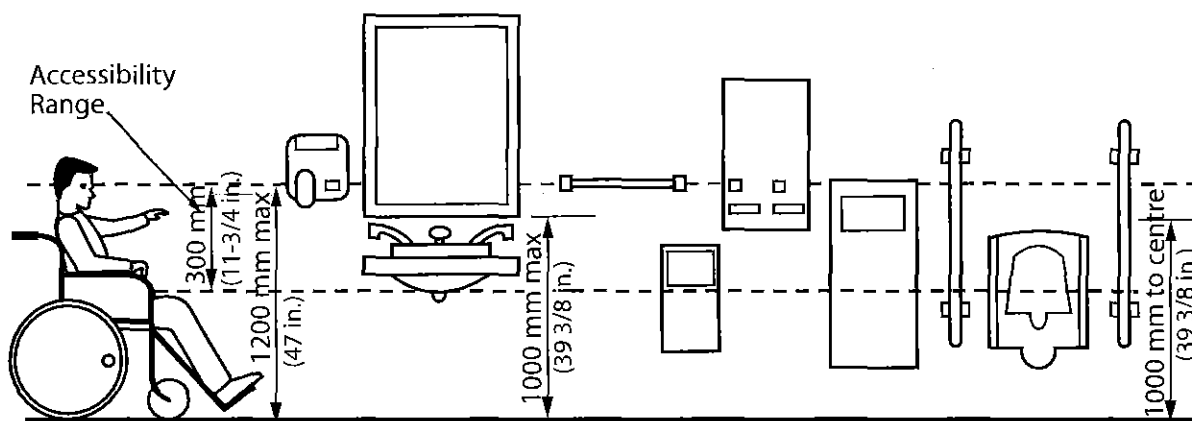
Figure 4.2.6.1 Washroom Accessories
