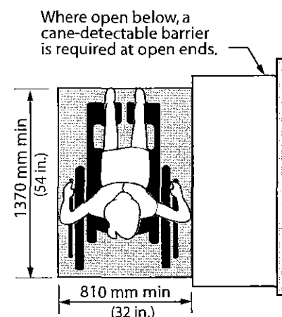
Figure 4.3.7.3 Parallel Approach
