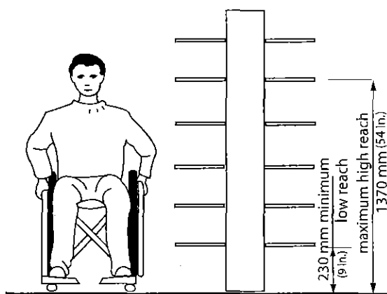
Figure 4.5.6.2 Reach Heights
