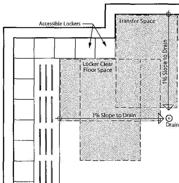
Figure 4.3.10.1 Locker Room Clear Floor Space requirements
