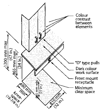
Figure 4.3.18.4 Storage Elements
