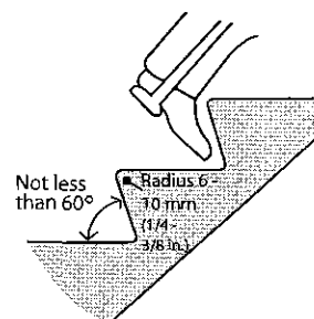
Figure 4.1.11.3 Raked Riser
