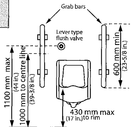
Figure 4.2.5.2 Urinal
