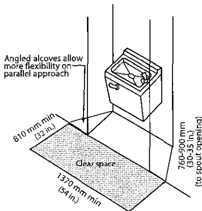
Figure 4.3.1.1 Parallel Approach
