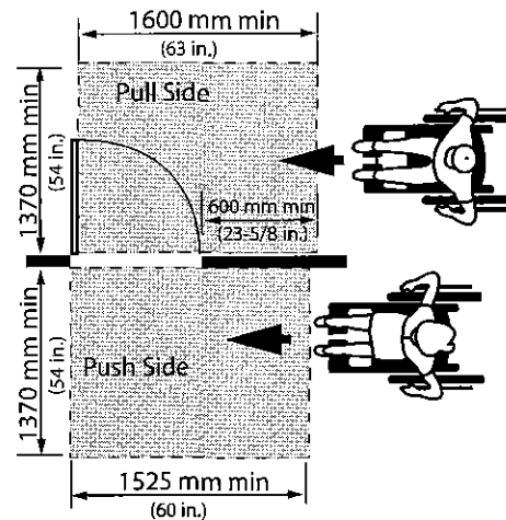
Figure 4.1.6.2 Latch Side Approach at Hinged Doors
