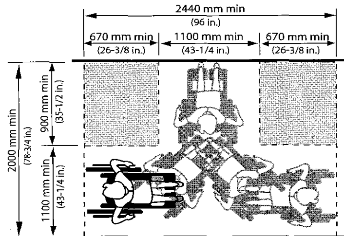
Figure 4.1.1.2 180° Turning Space
