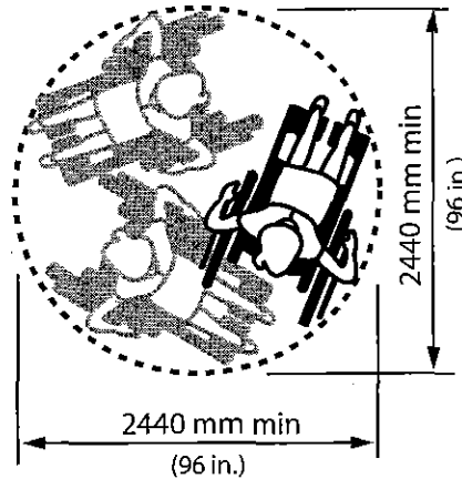
Figure 4.1.1.1 360° Turning Space
