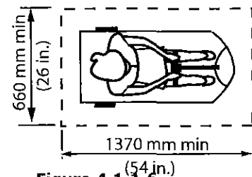
Figure 4.1.1.6 Clear Floor Space for Scooter
