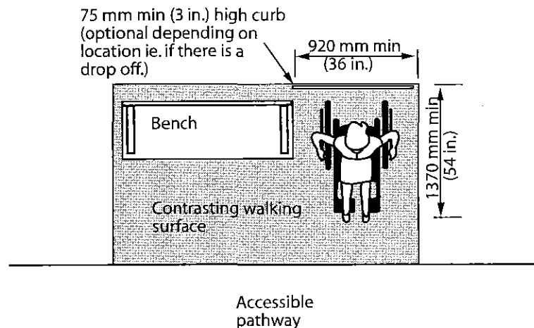
Figure 4.3.15.1 Rest Area
