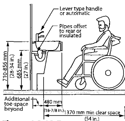
Figure 4.3.18.5 Kitchen Sink
