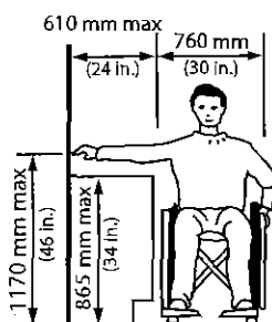
Figure 4.1.1.10 Side Reach over an Obstruction
