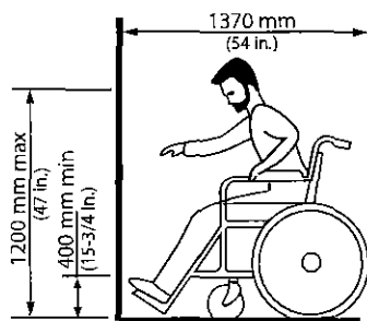
Figure 4.1.1.11 Forward Reach
