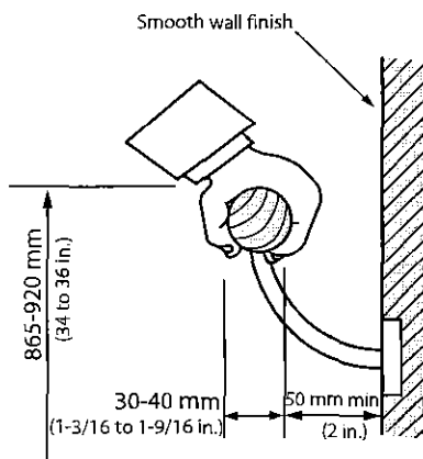
Figure 4.1.12.1 Handrail
