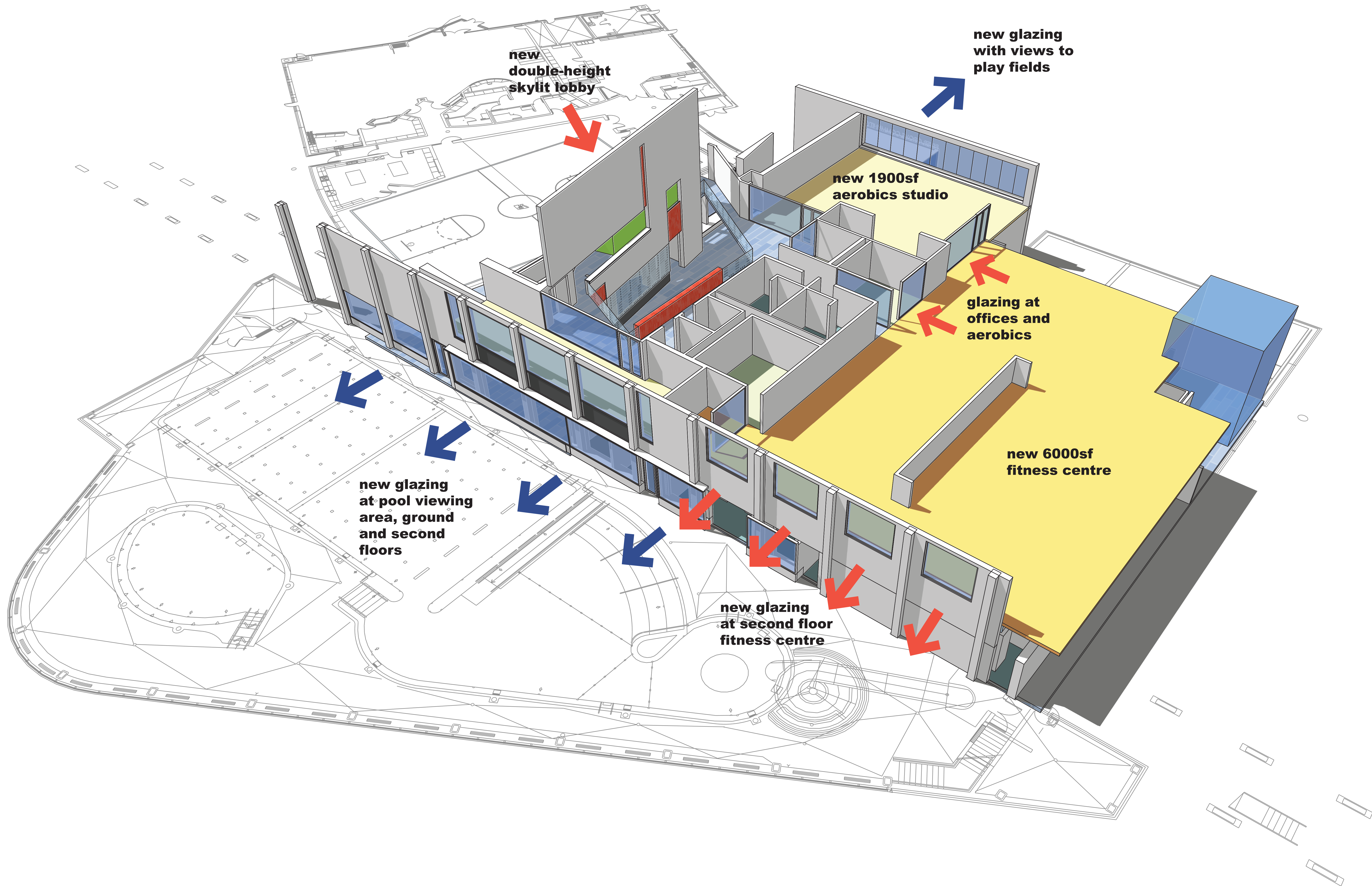
AERIAL VIEW - SECOND FLOOR RIVER GROVE COMMUNITY CENTRE RENOVATION may 2013: renovated area shown in colour, existing plan shown in grey
