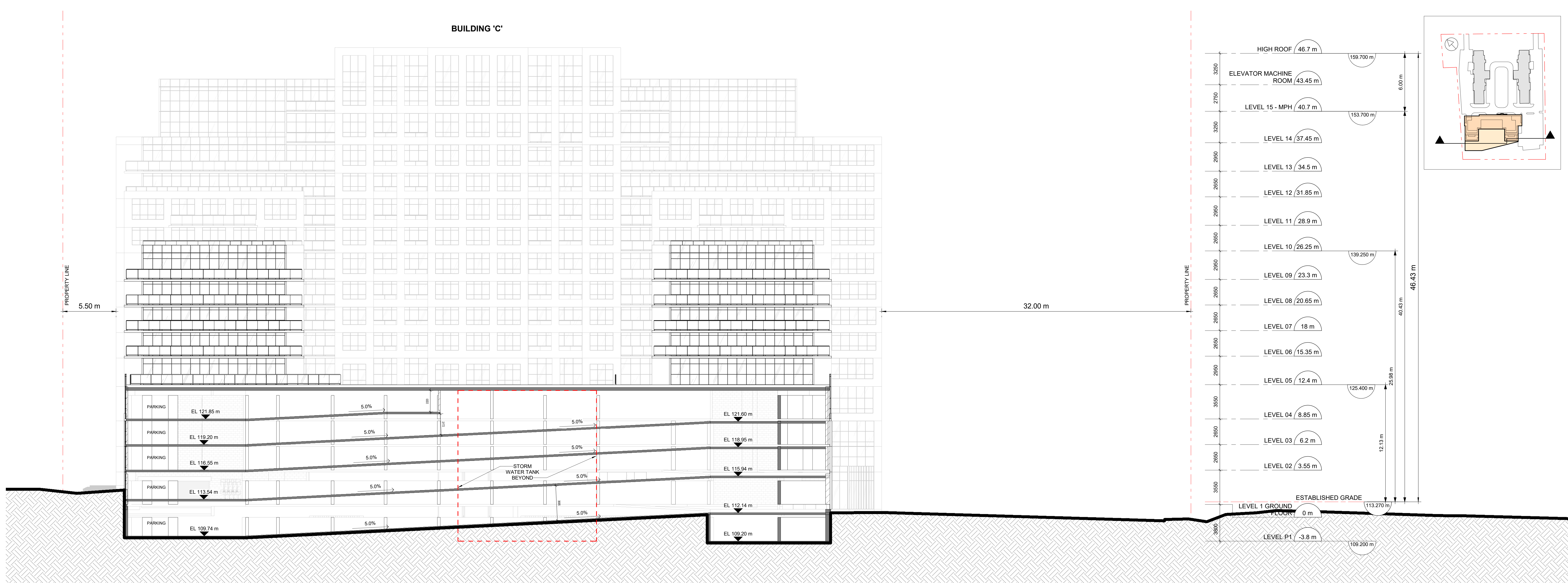
2 NORTH-SOUTH RAMP SECTION A-302 Scale: 1:150
