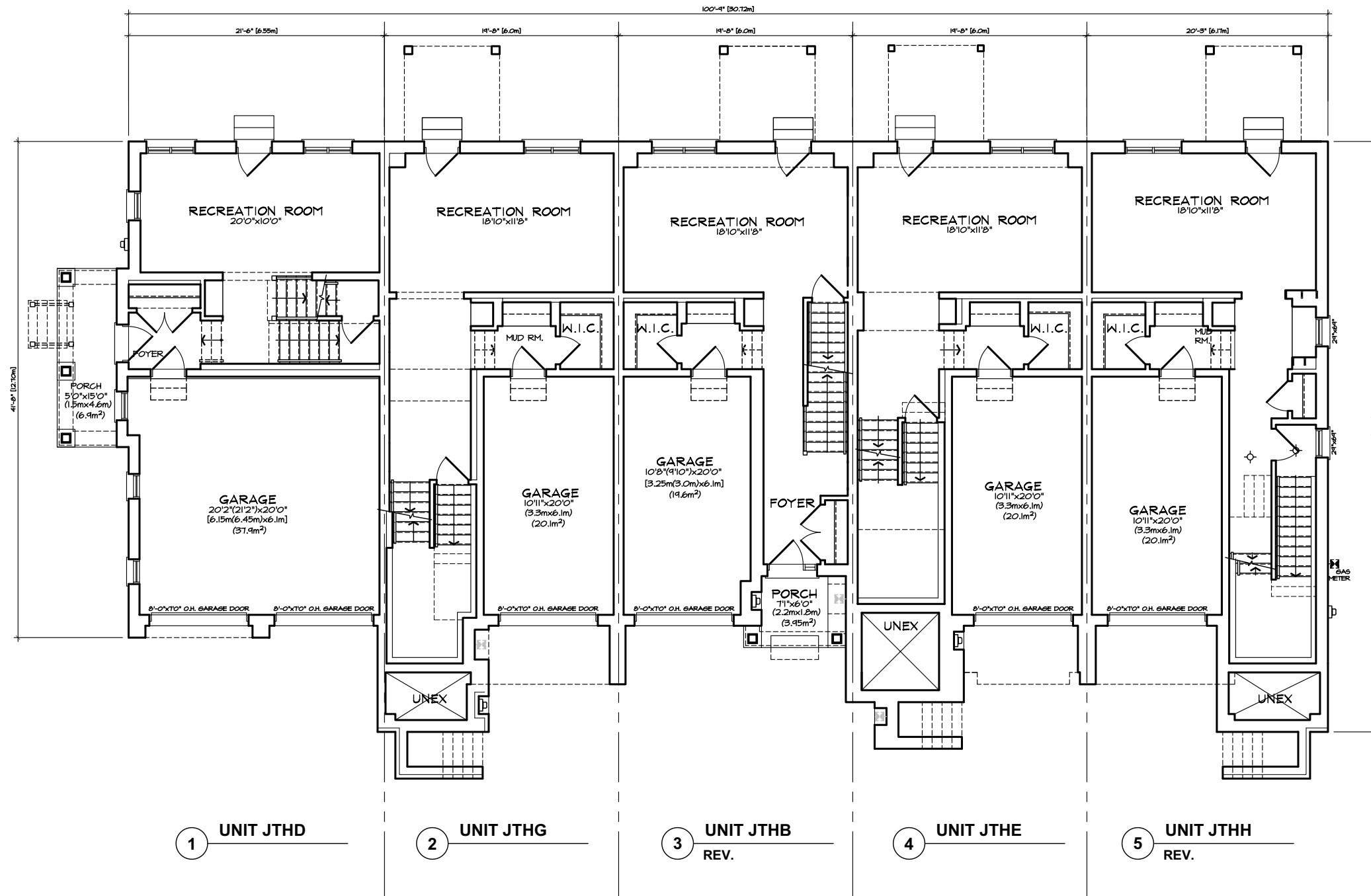
GROUND FLOOR PLAN 'TA' FRONT LOAD TOWNS BLOCK 4
