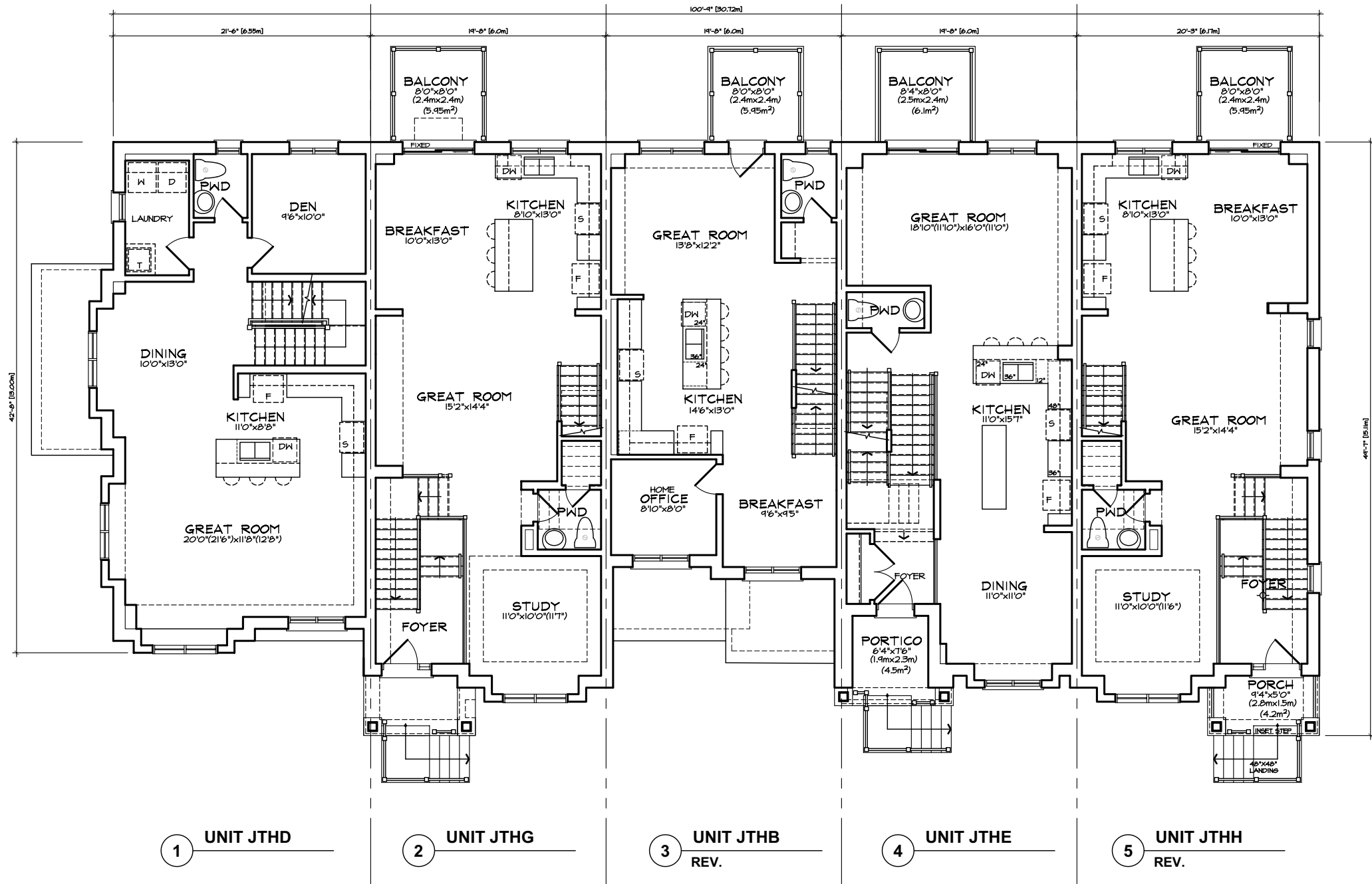
MAIN FLOOR PLAN 'TA' FRONT LOAD TOWNS BLOCK 4
