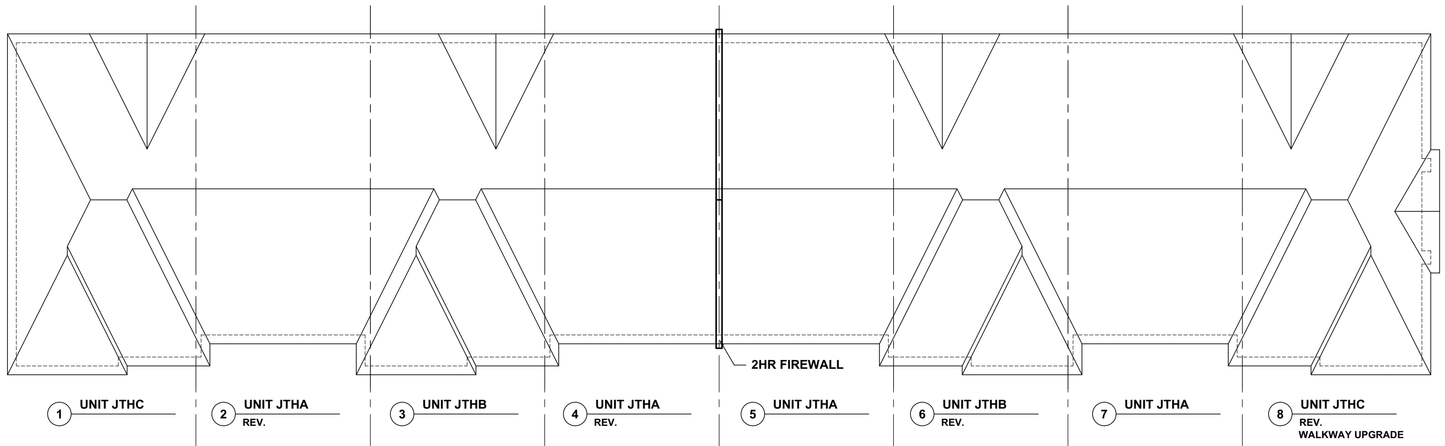
ROOF PLAN 'TA' FRONT LOAD TOWNS BLOCK 17
