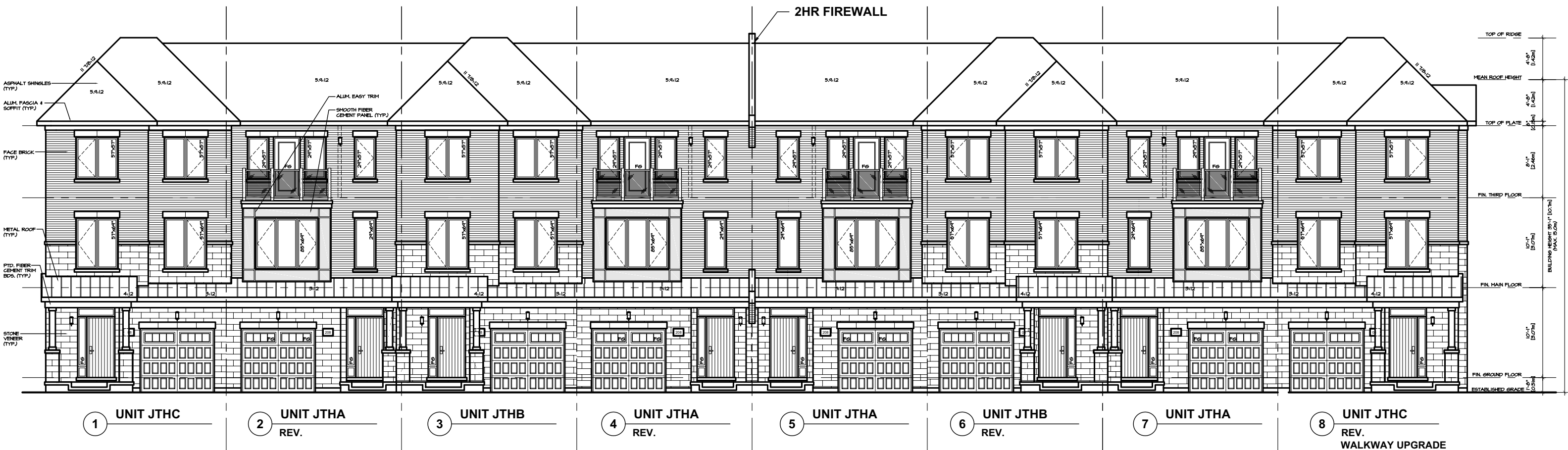
SOUTH ELEVATION 'TA' FRONT LOAD TOWNS BLOCK 17
