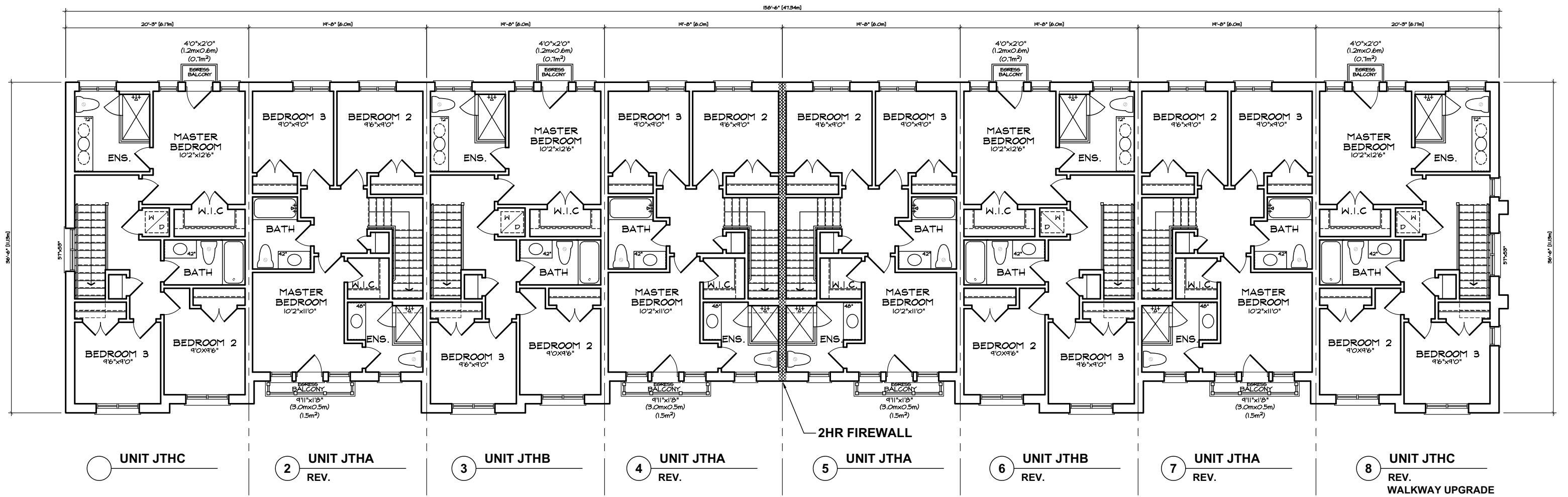
THIRD FLOOR PLAN 'TA' FRONT LOAD TOWNS BLOCK 17
