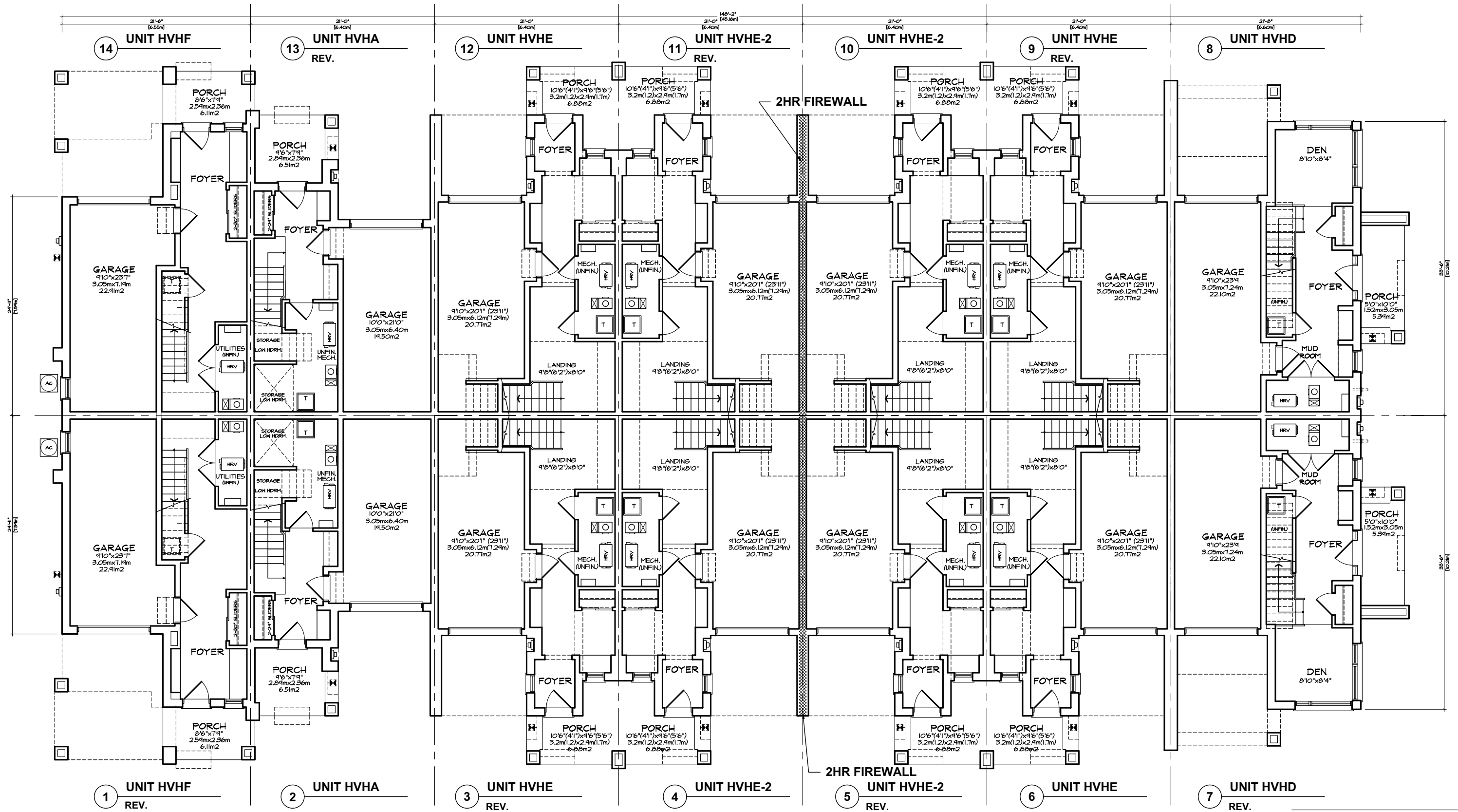
GROUND FLOOR PLAN 'MO' VILLAGE HOMES BLOCK 15
