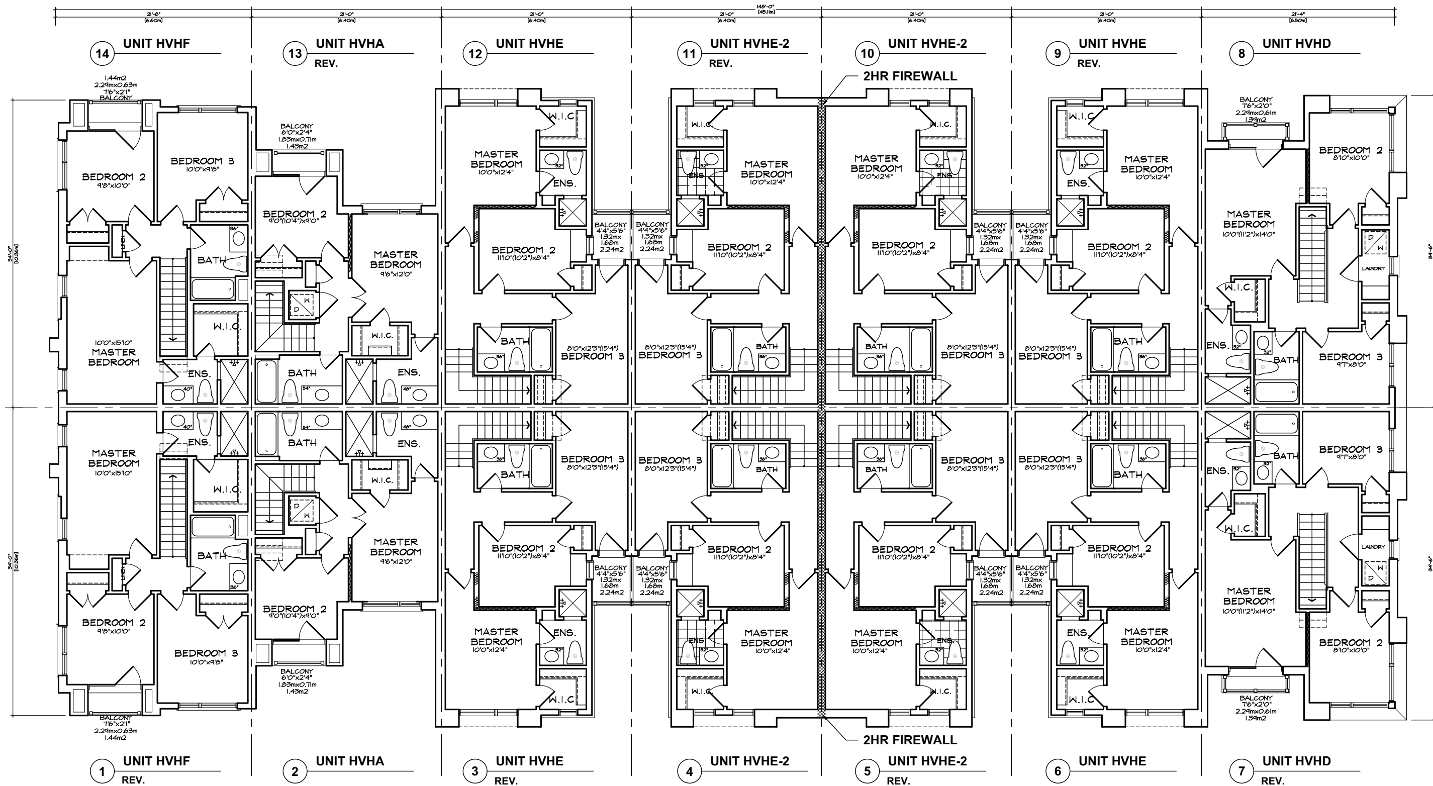
THIRD FLOOR PLAN 'MO' VILLAGE HOMES BLOCK 15
