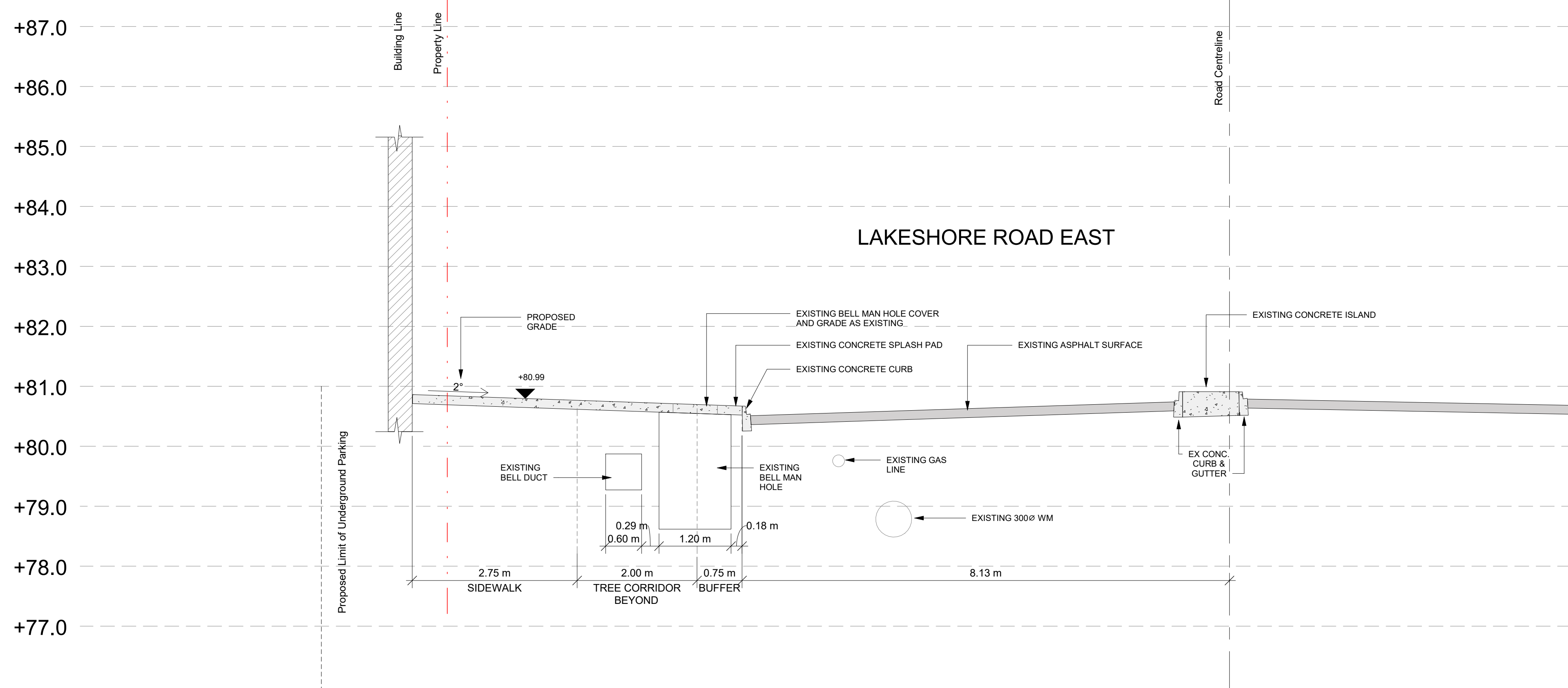
PROPOSED SECTION A-A - LAKESHORE ROAD EAST
