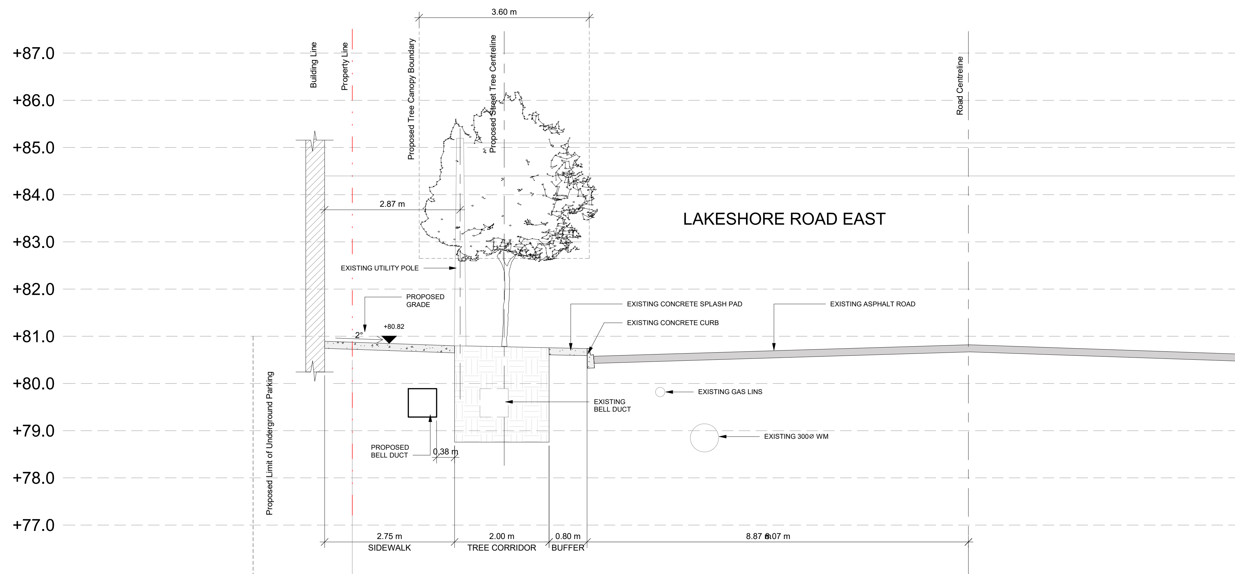
PROPOSED SECTION B-B - LAKESHORE ROAD EAST
