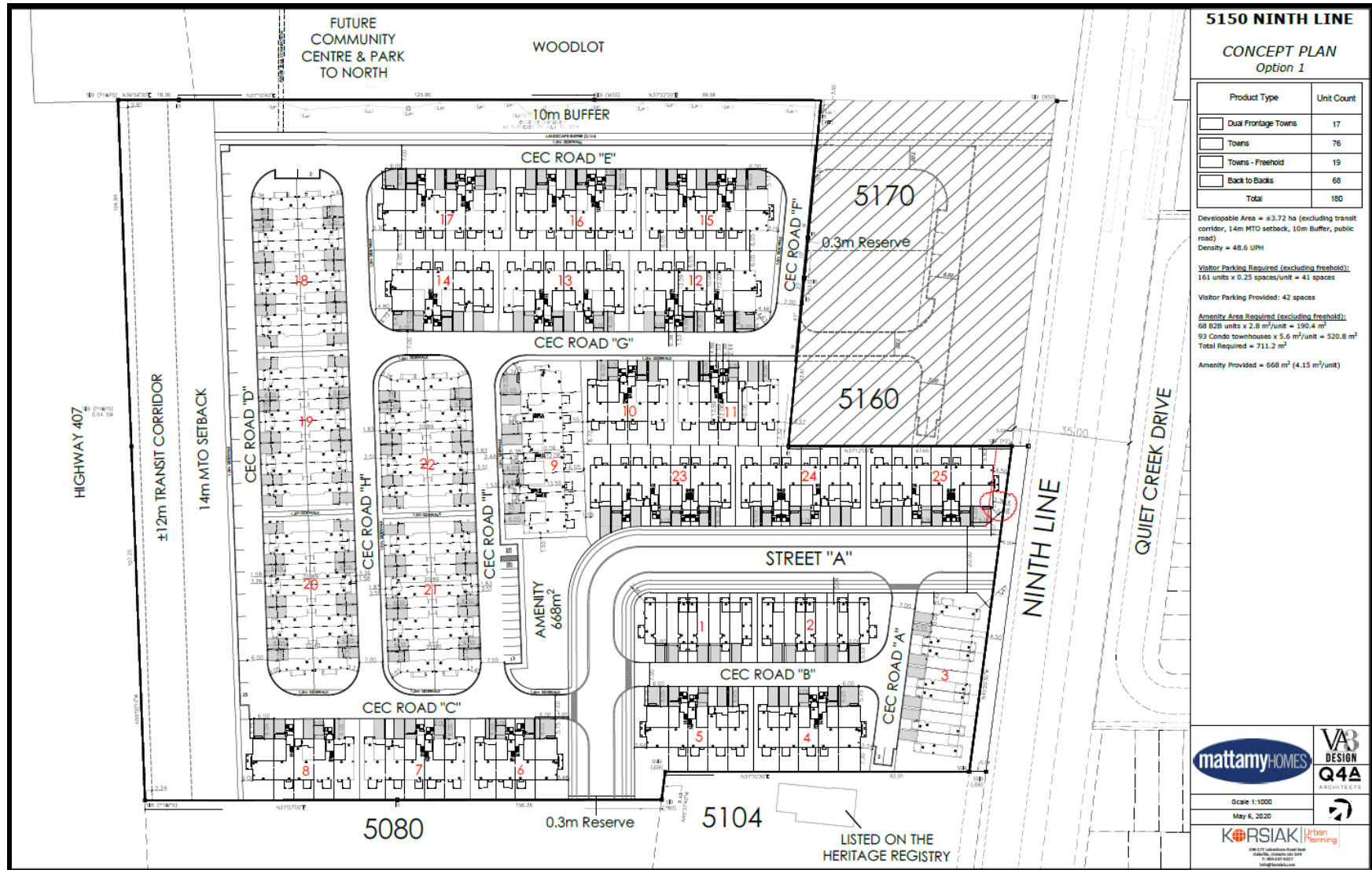
Figure 3: Concept Plan for 5150 Ninth Line (Mattamy 2020)
