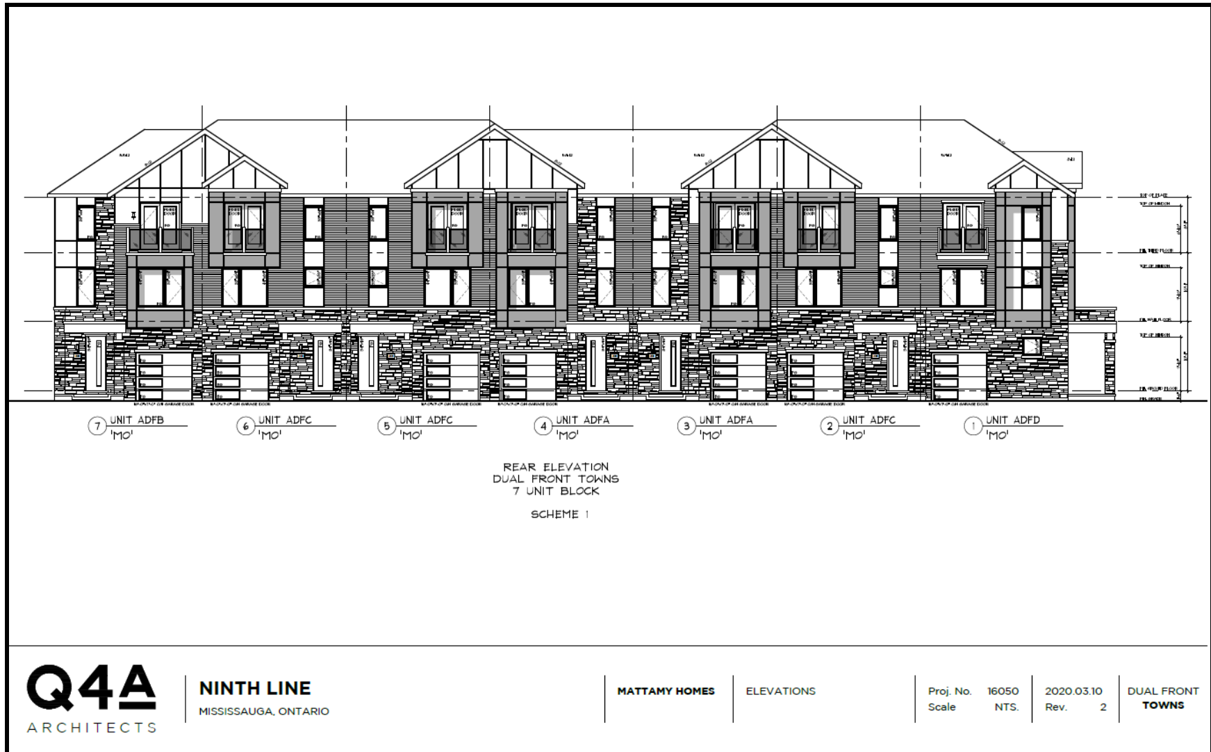
Figure 8: Dual Front Towns, 7 Unit Block – Rear Elevation (Scheme 1) (Q4A Architects 2020)
