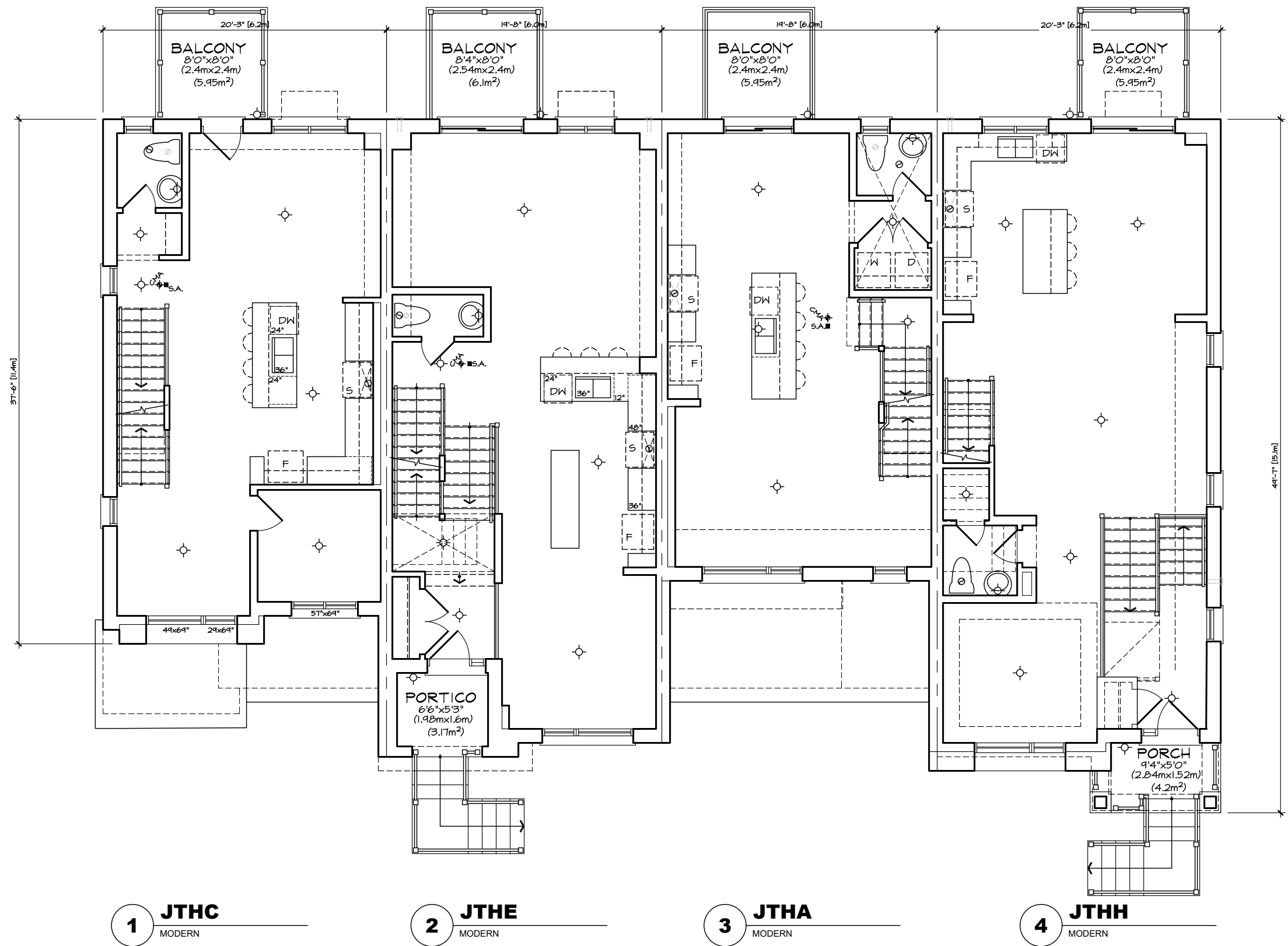
MAIN FLOOR PLAN 'MO' FRONT LOAD TOWN BLOCK 2
