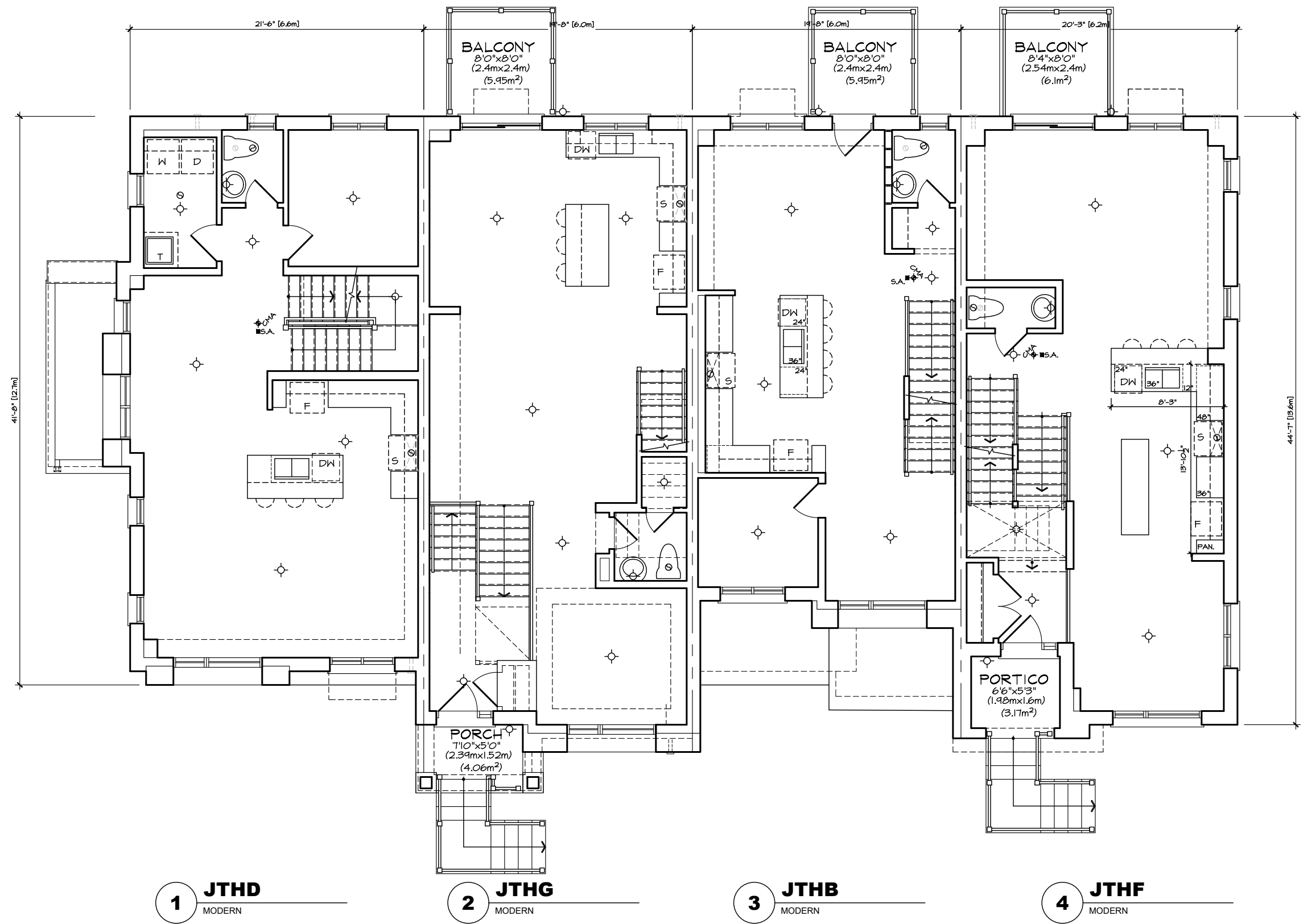
MAIN FLOOR PLAN 'MO' FRONT LOAD TOWN BLOCK 1
