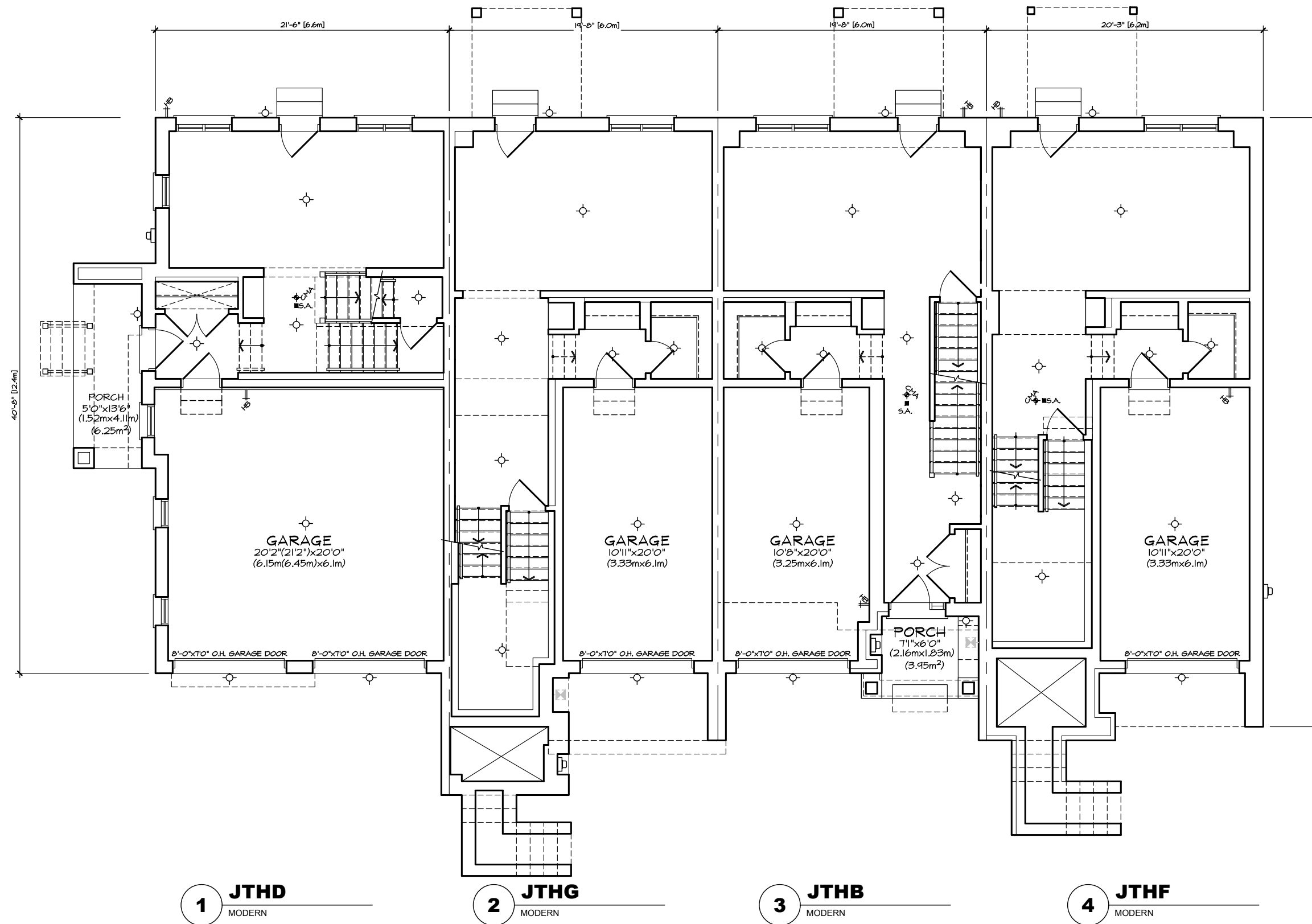
GROUND FLOOR PLAN 'MO' FRONT LOAD TOWN BLOCK 1
