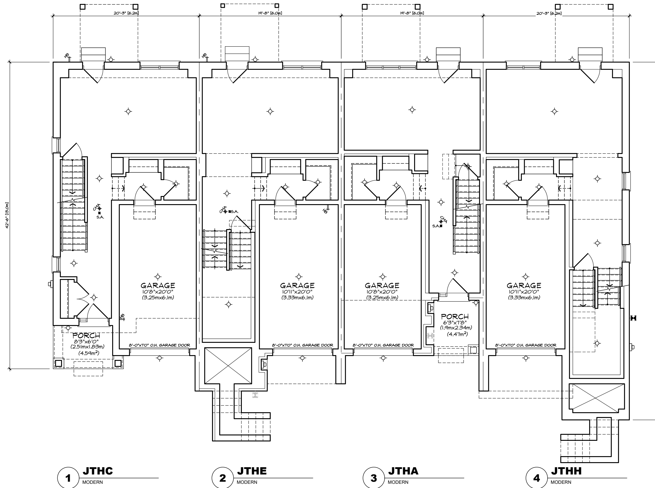
GROUND FLOOR PLAN 'MO' FRONT LOAD TOWN BLOCK 2
