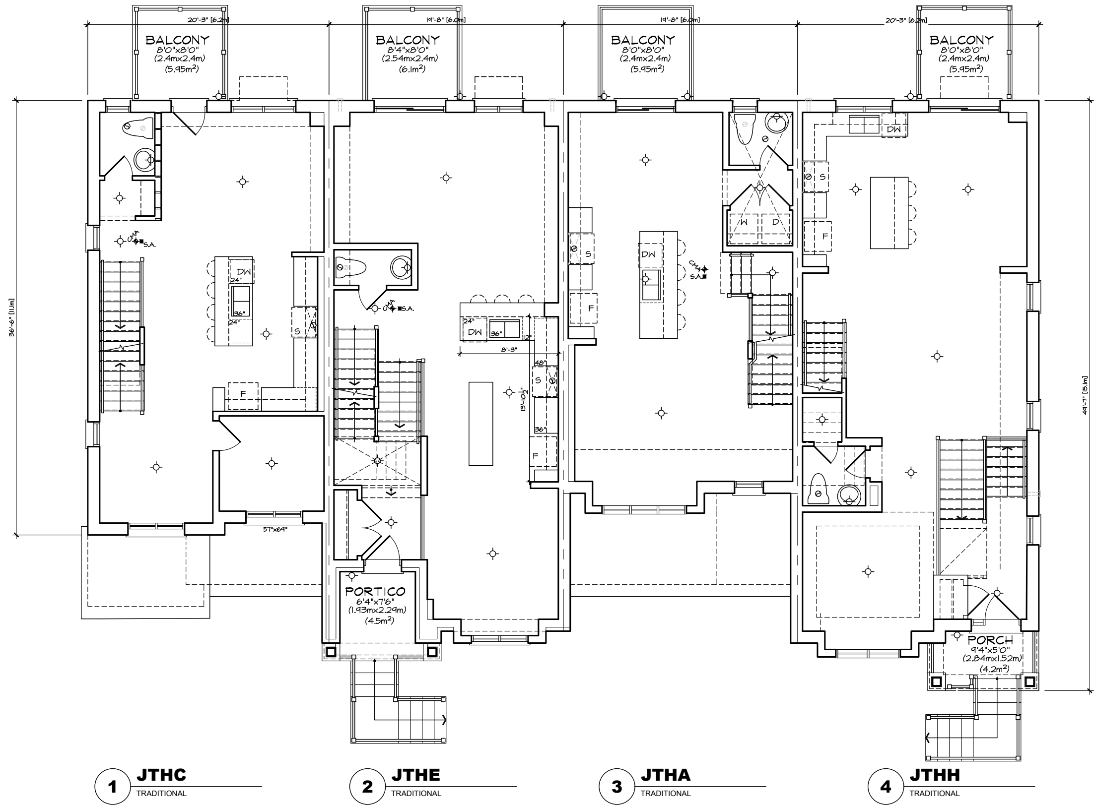
MAIN FLOOR PLAN 'TA' FRONT LOAD TOWN BLOCK 2
