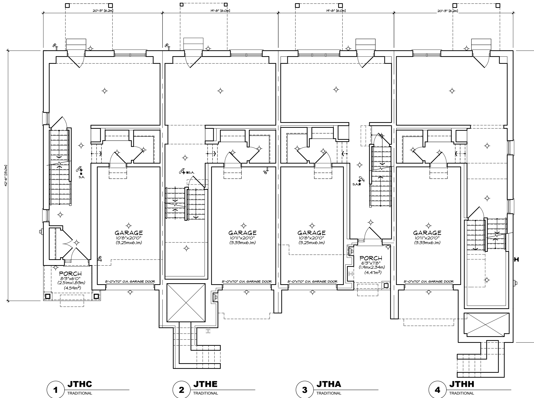
GROUND FLOOR PLAN 'TA' FRONT LOAD TOWN BLOCK 2
