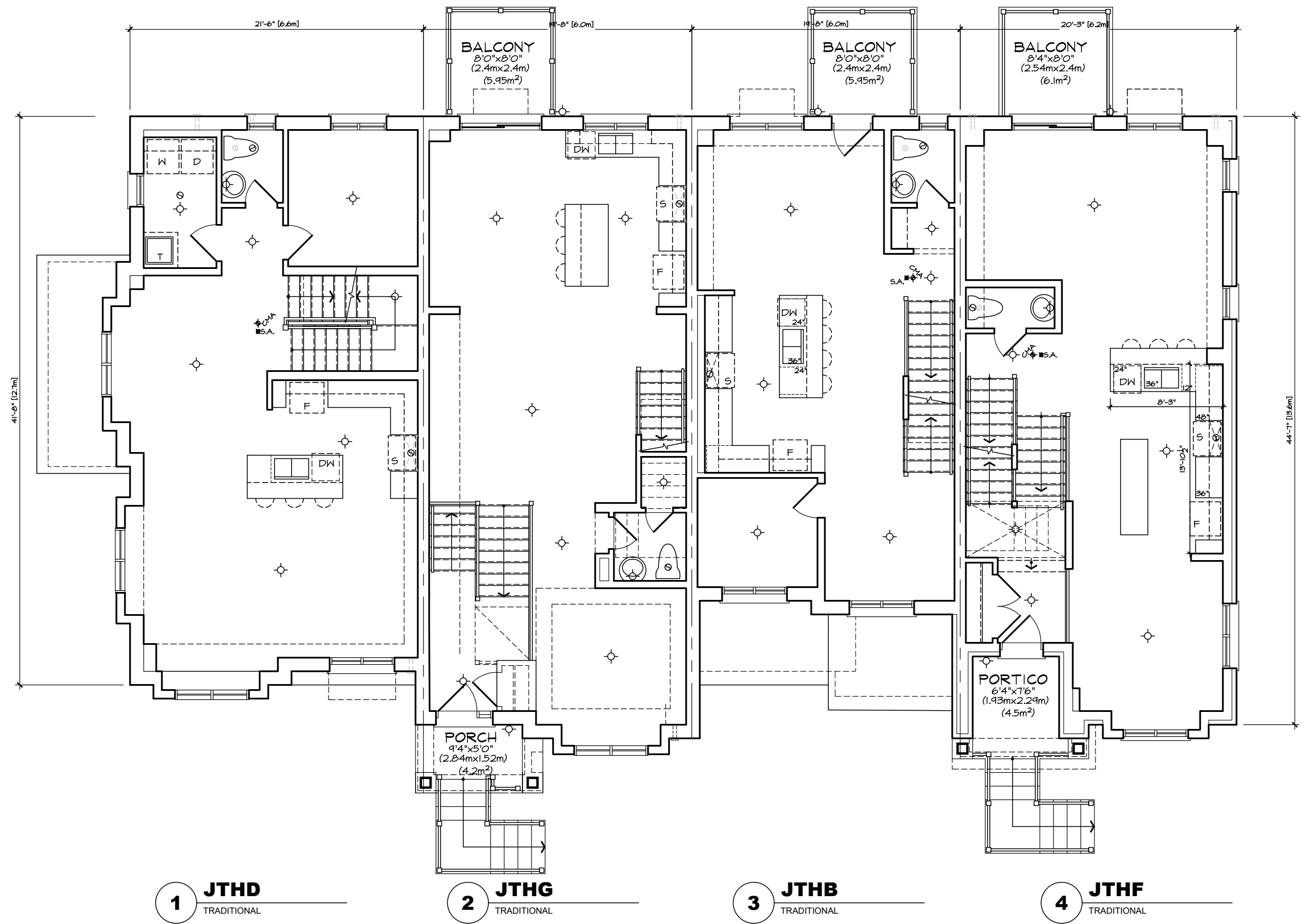
MAIN FLOOR PLAN 'TA' FRONT LOAD TOWN BLOCK 1
