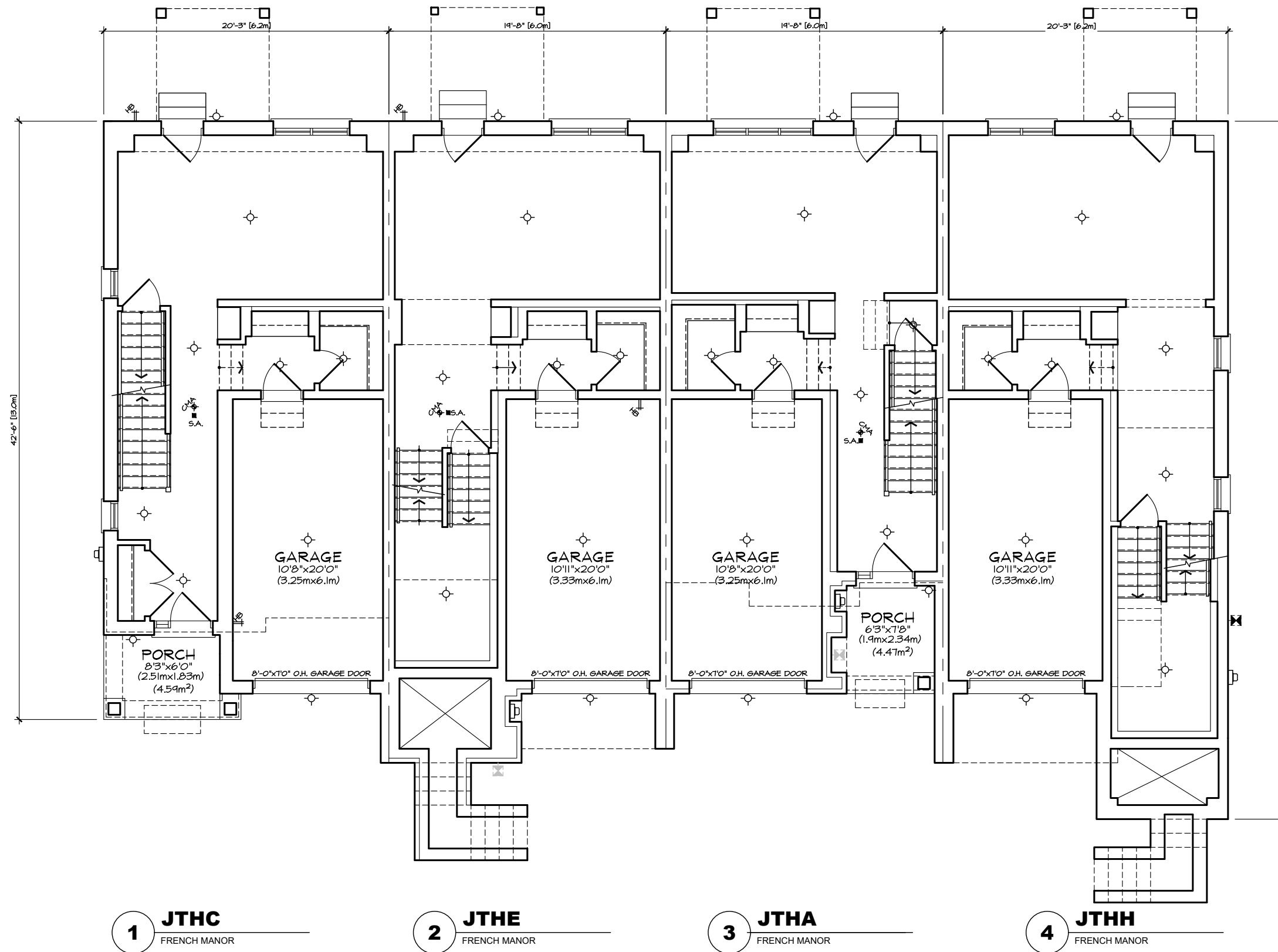
GROUND FLOOR PLAN 'FM' FRONT LOAD TOWN BLOCK 2
