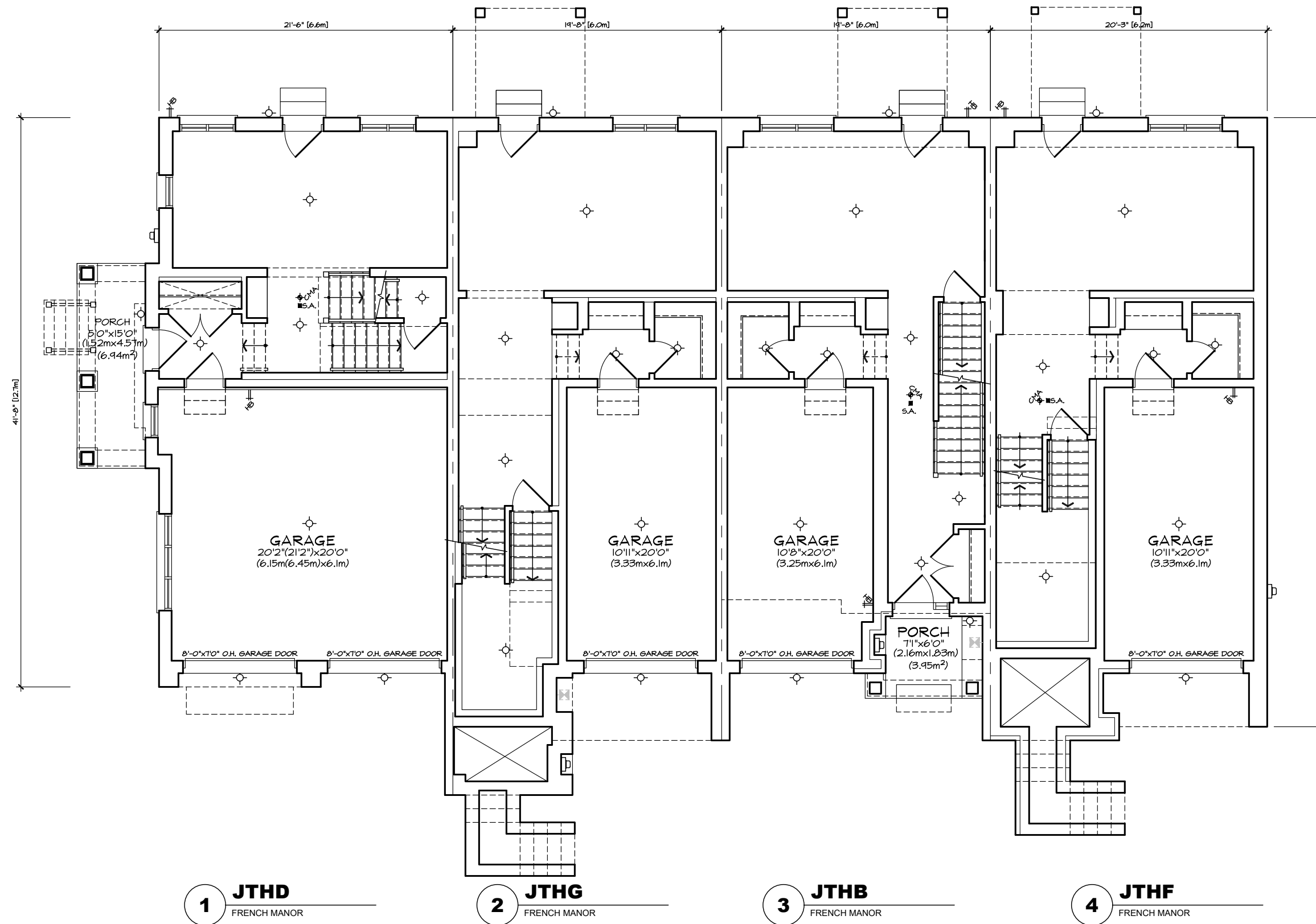
GROUND FLOOR PLAN 'FM' FRONT LOAD TOWN BLOCK 1
