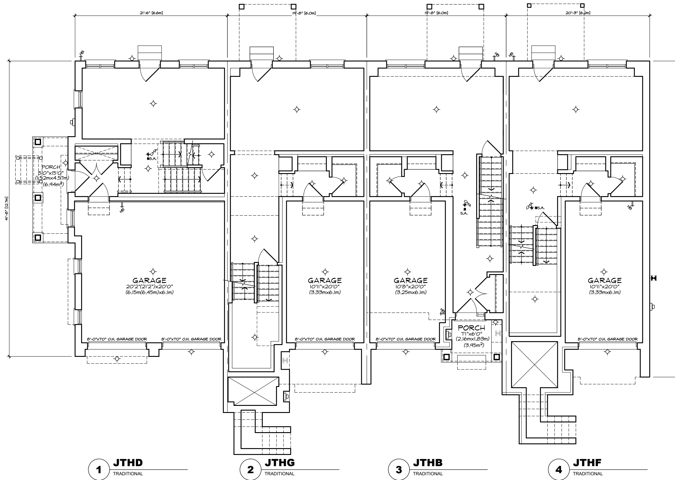
GROUND FLOOR PLAN 'TA' FRONT LOAD TOWN BLOCK 1
