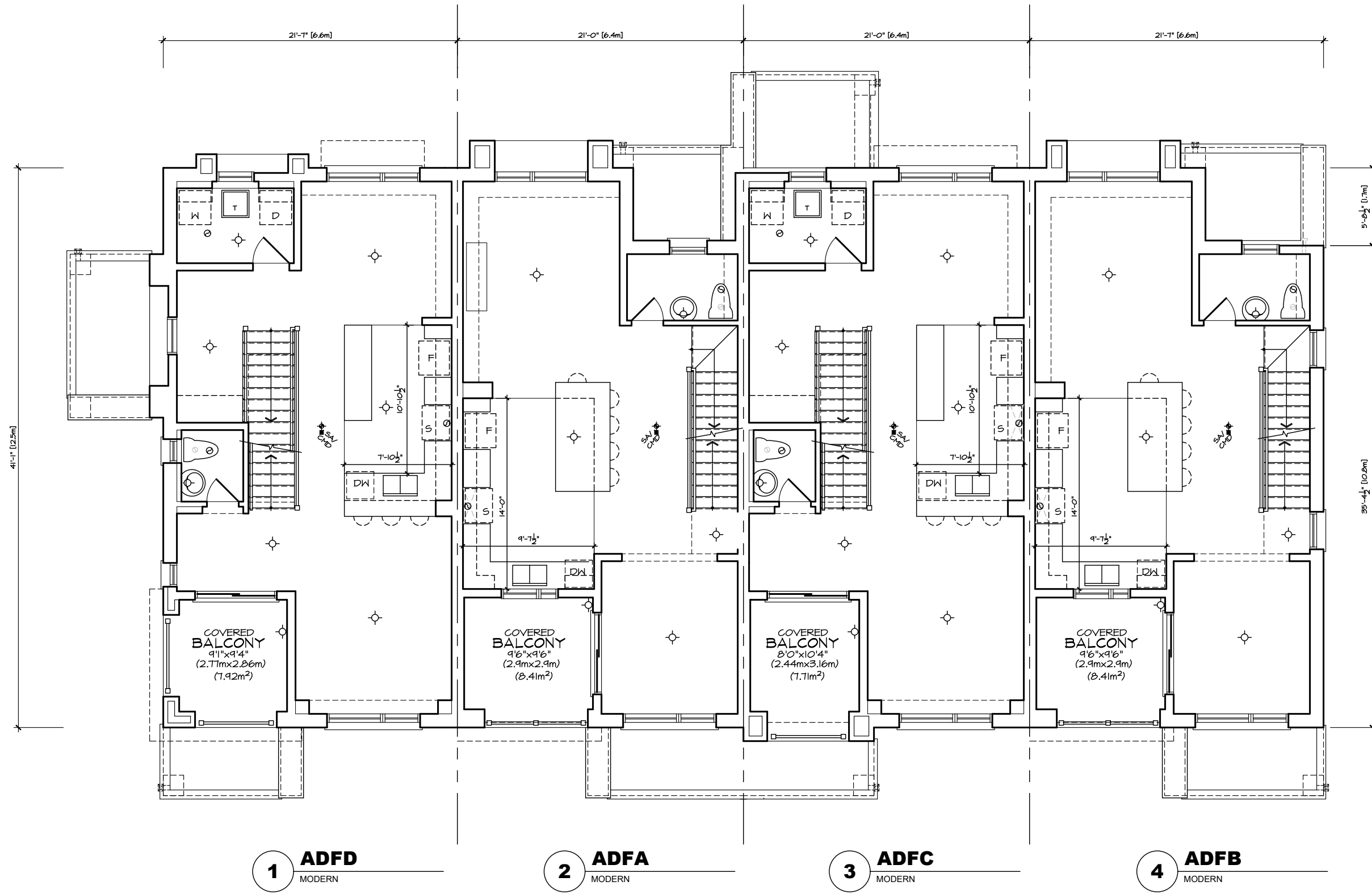
MAIN FLOOR PLAN 'MO' DUAL FRONT TOWNS
