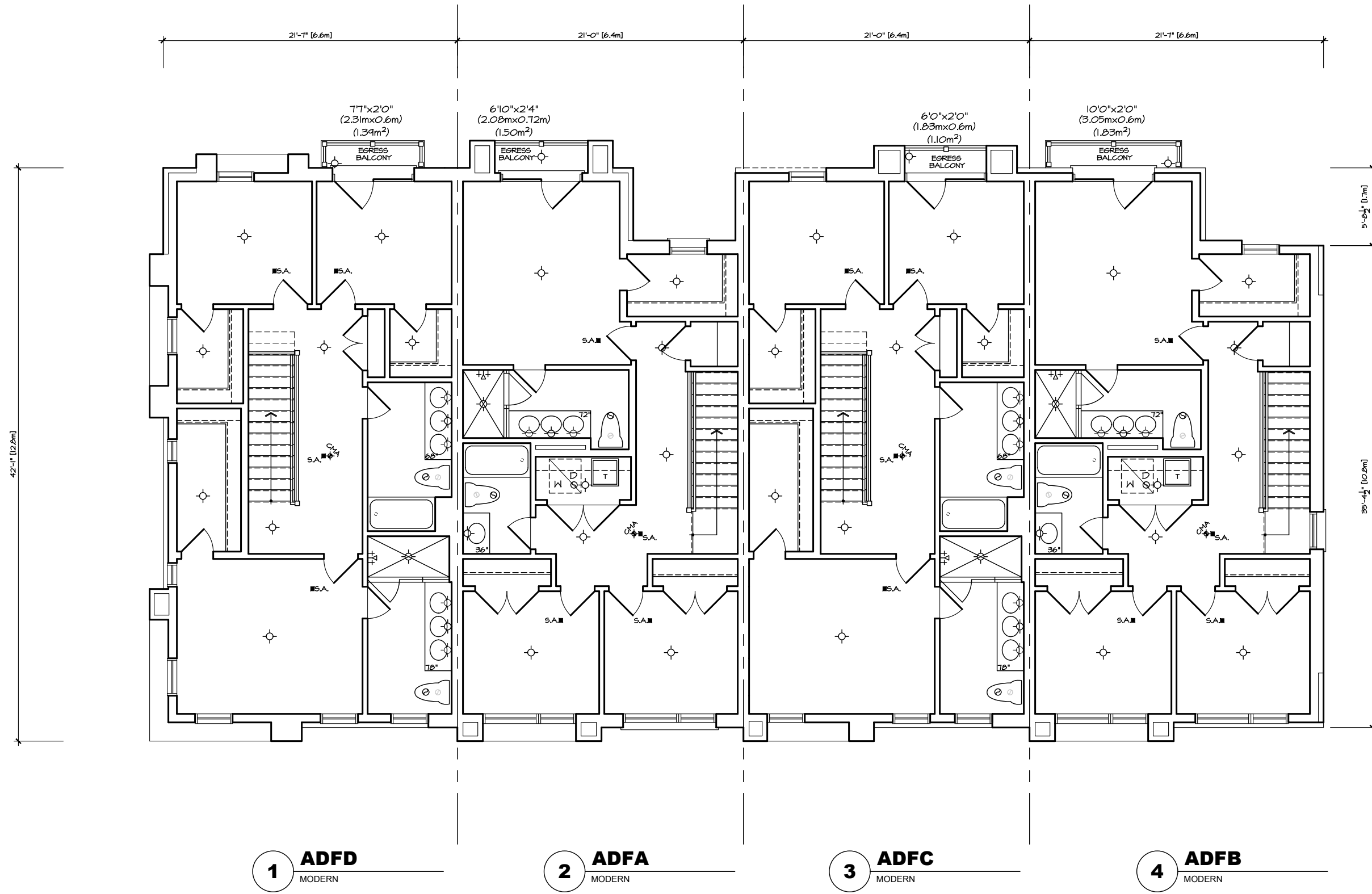
THIRD FLOOR PLAN 'MO' DUAL FRONT TOWNS
