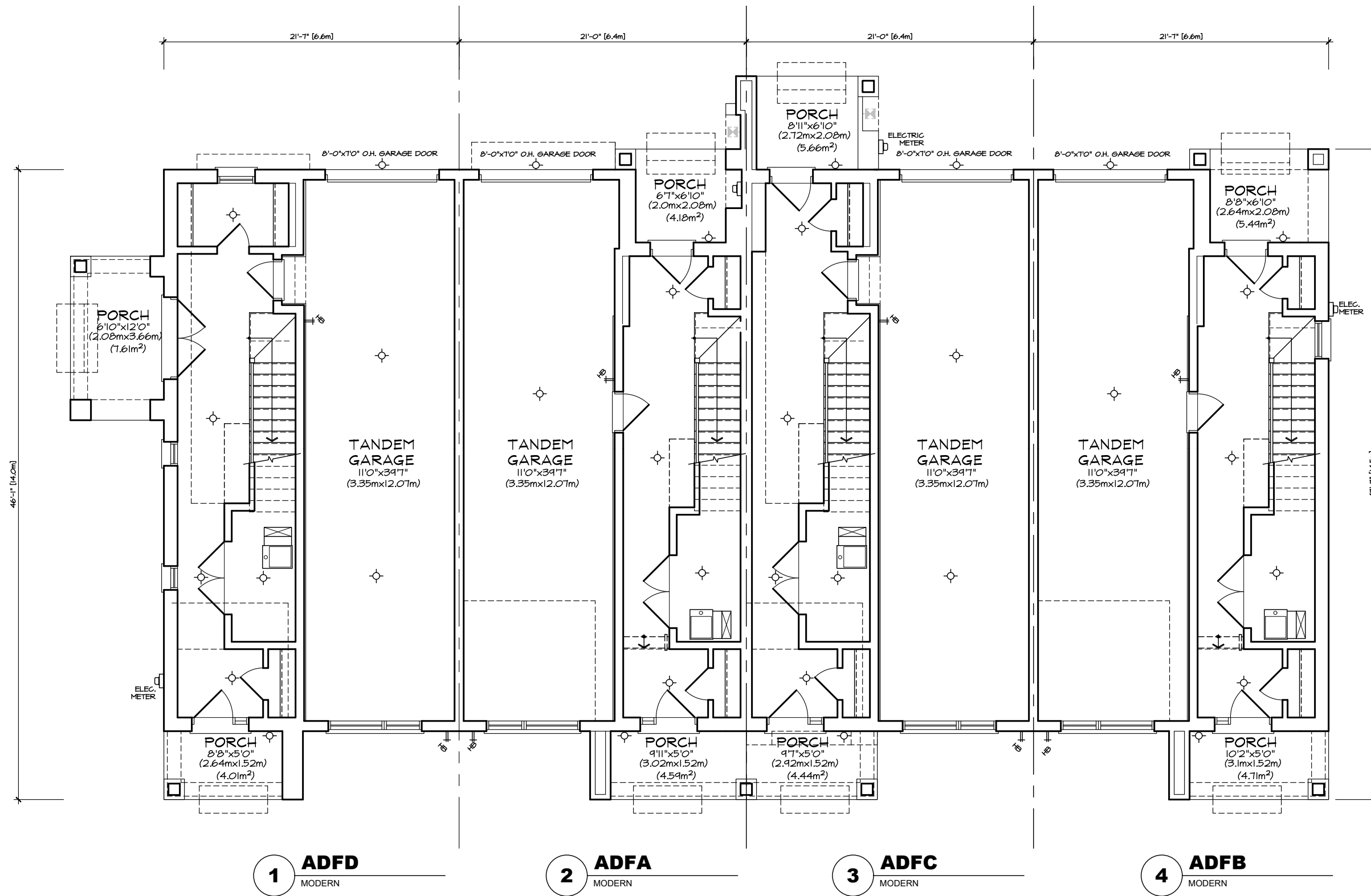
GROUND FLOOR PLAN 'MO' DUAL FRONT TOWNS
