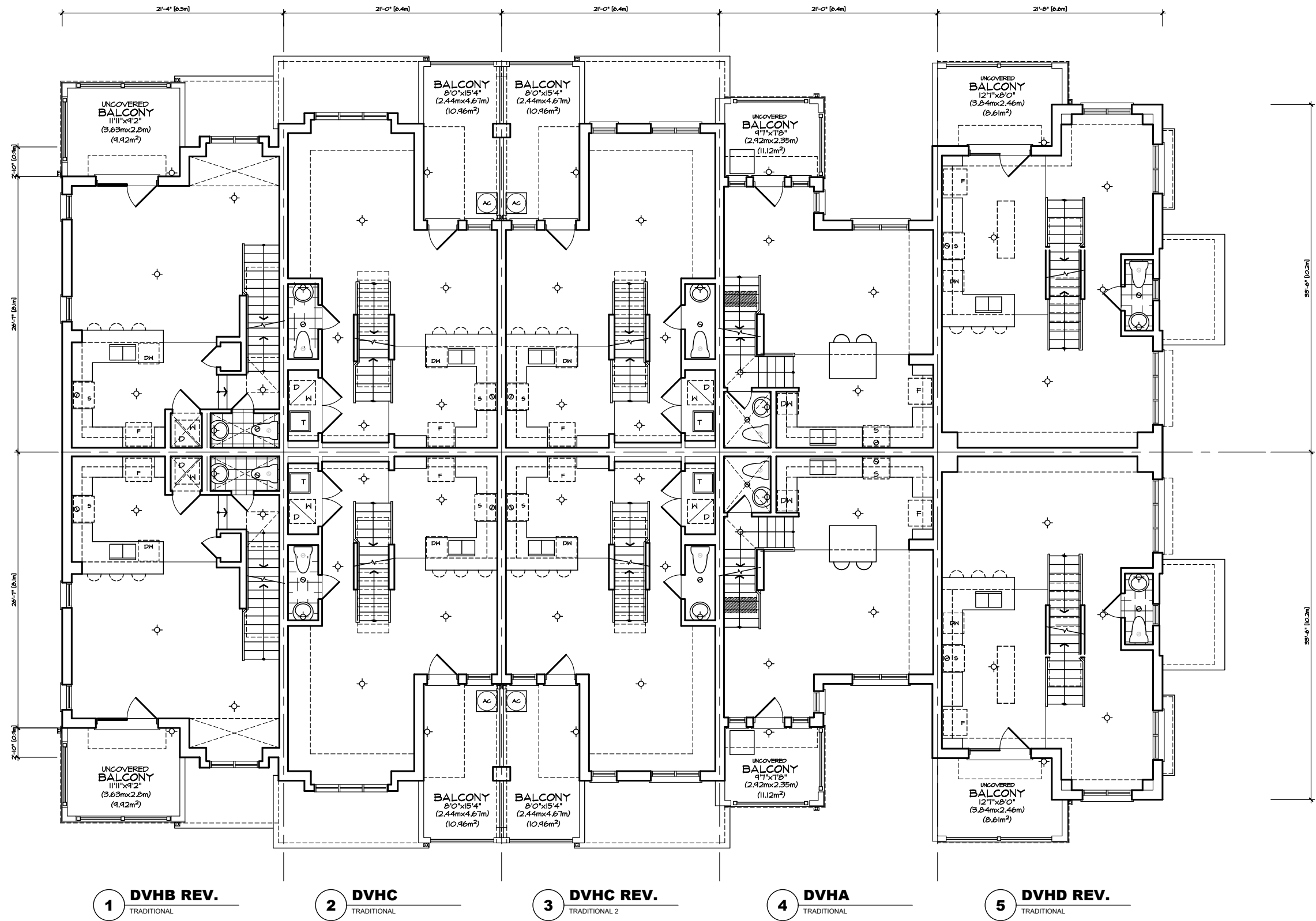
MAIN FLOOR PLAN 'TA' VILLAGE HOMES BLOCK 2
