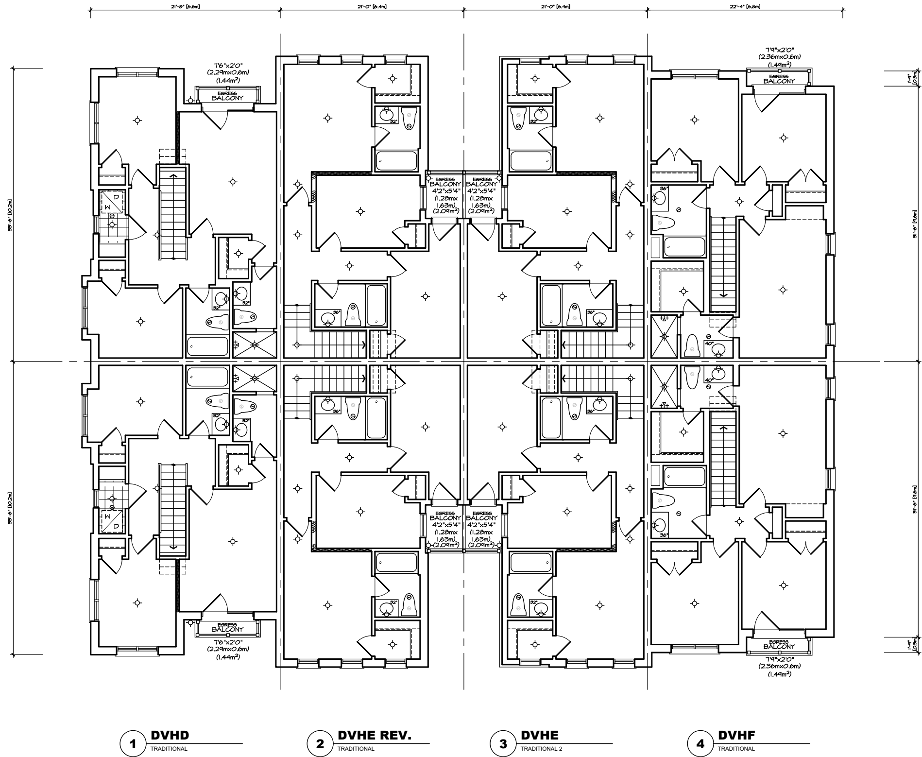
THIRD FLOOR PLAN 'TA' VILLAGE HOMES BLOCK 1
