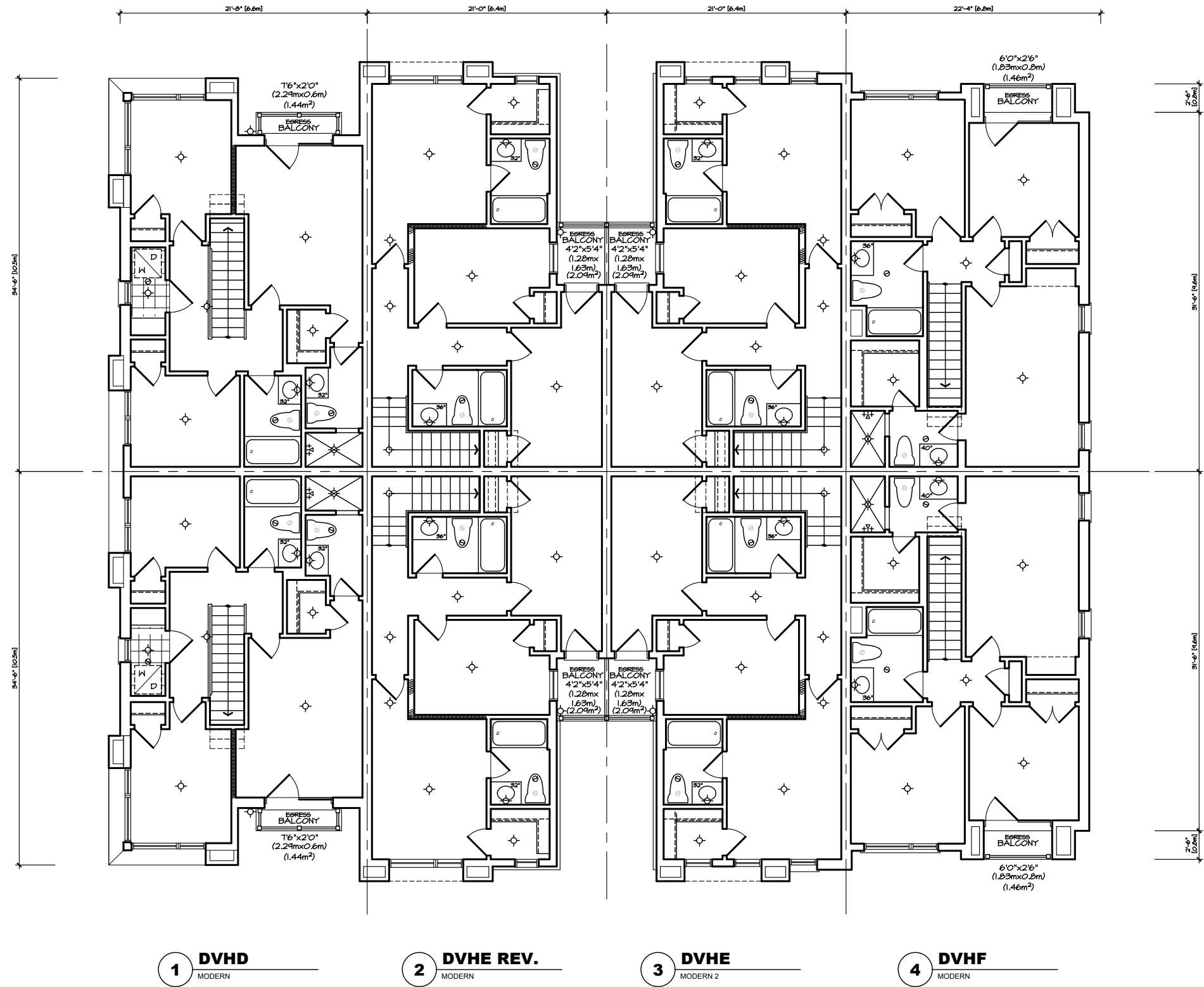
THIRD FLOOR PLAN 'MO' VILLAGE HOMES BLOCK 1
