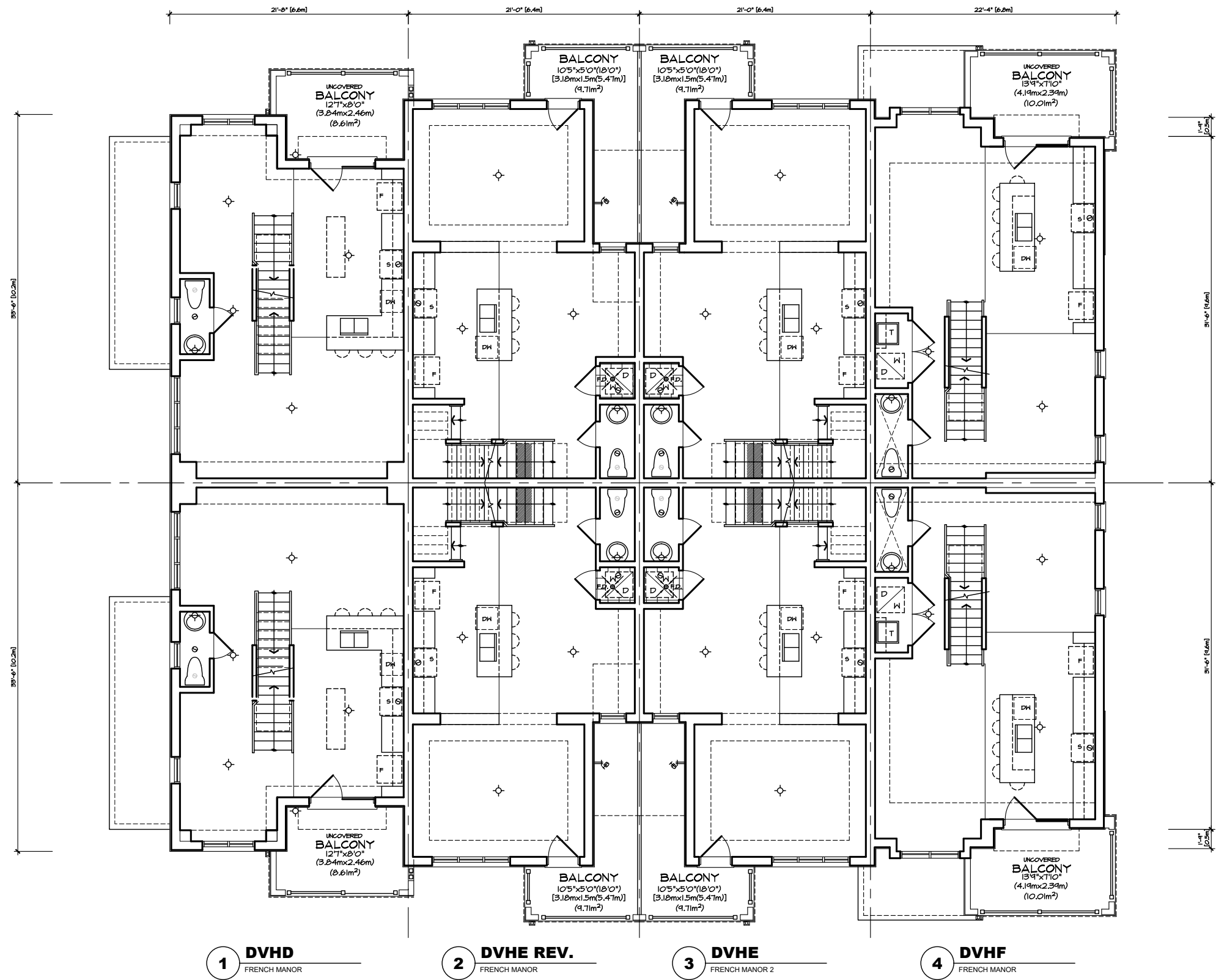
MAIN FLOOR PLAN 'FM' VILLAGE HOMES BLOCK 1
