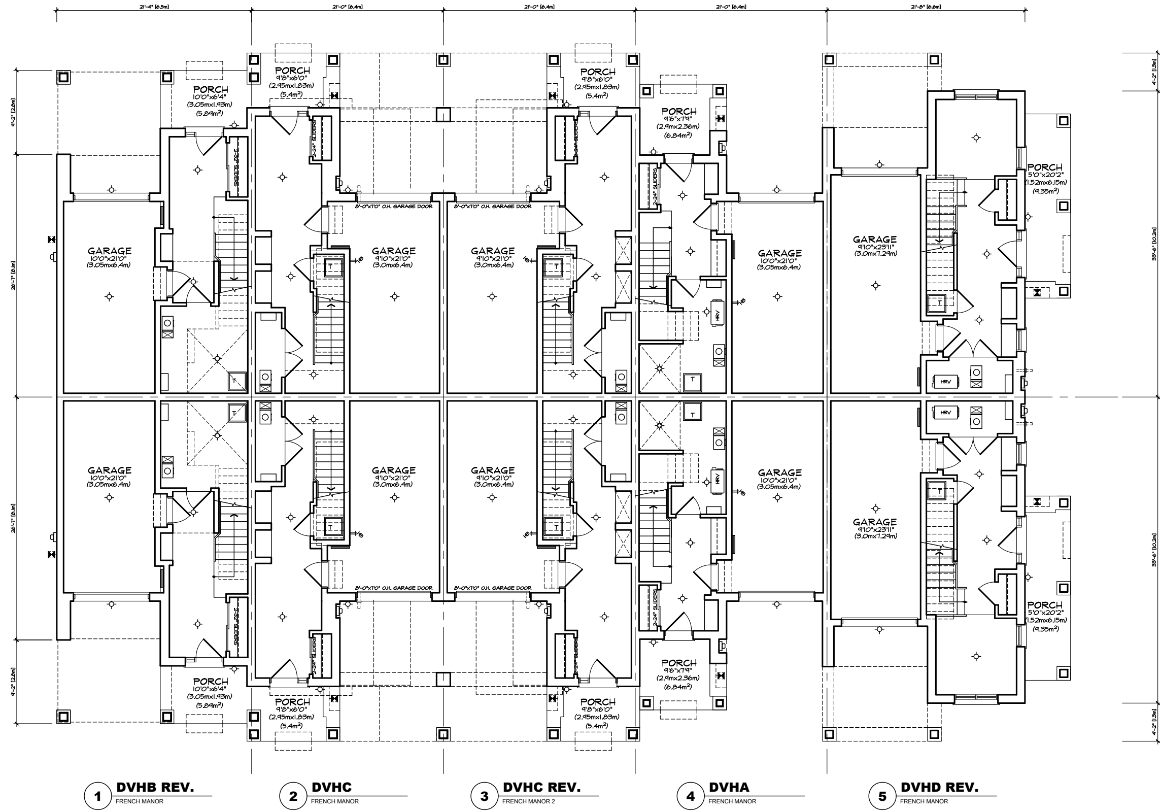
GROUND FLOOR PLAN 'FM' VILLAGE HOMES BLOCK 2
