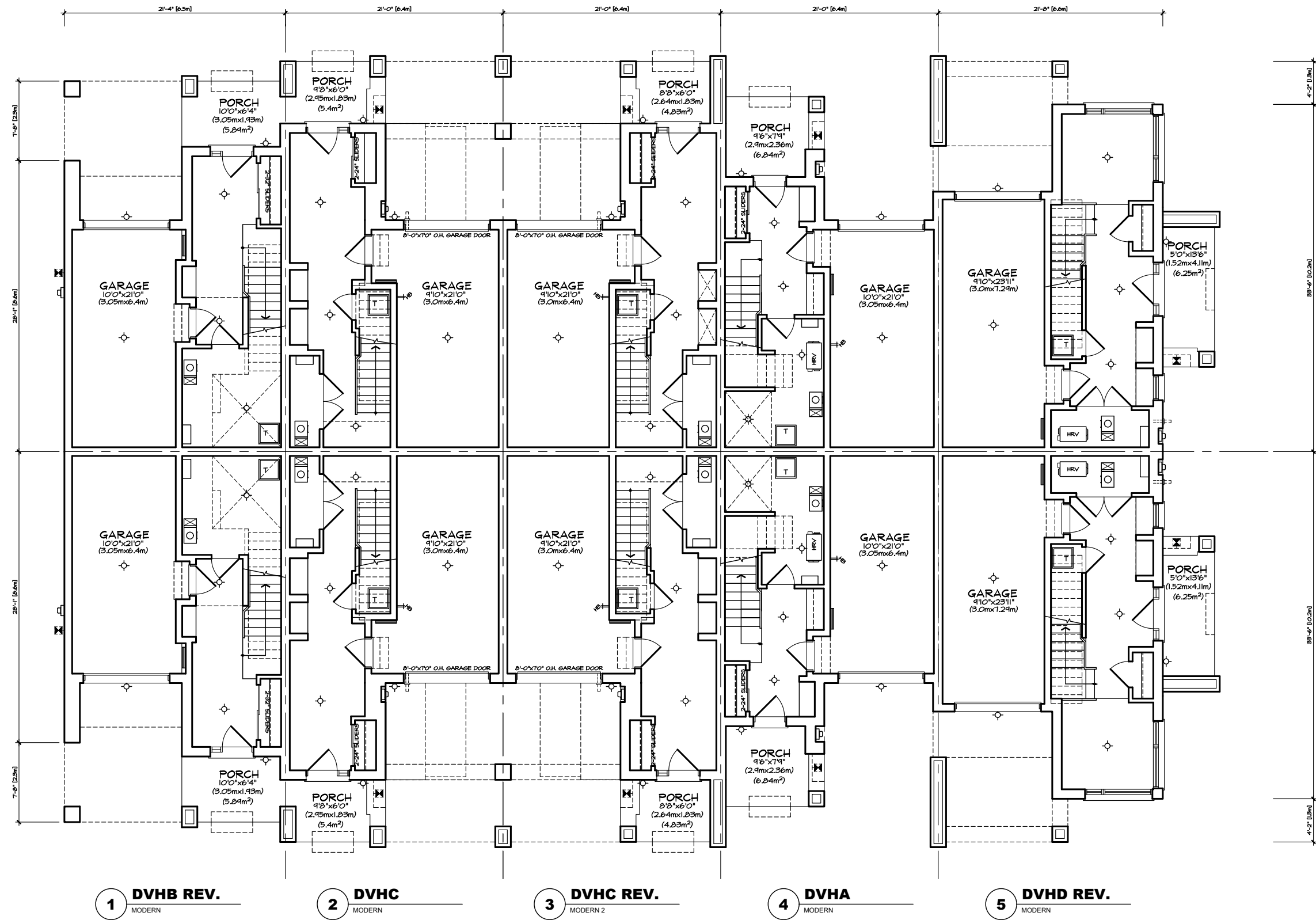
GROUND FLOOR PLAN 'MO' VILLAGE HOMES BLOCK 2
