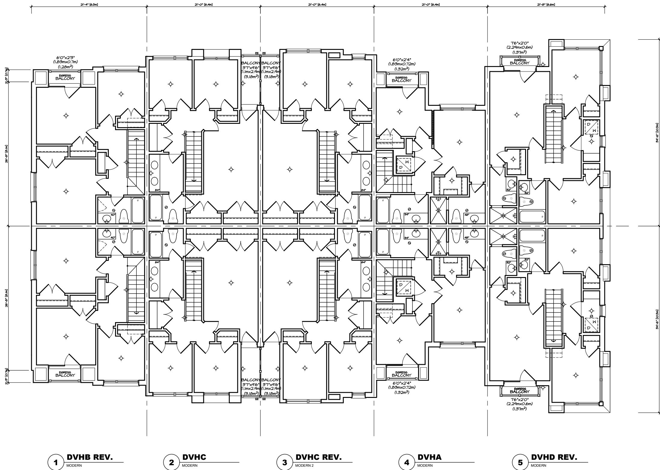
THIRD FLOOR PLAN 'MO' VILLAGE HOMES BLOCK 2
