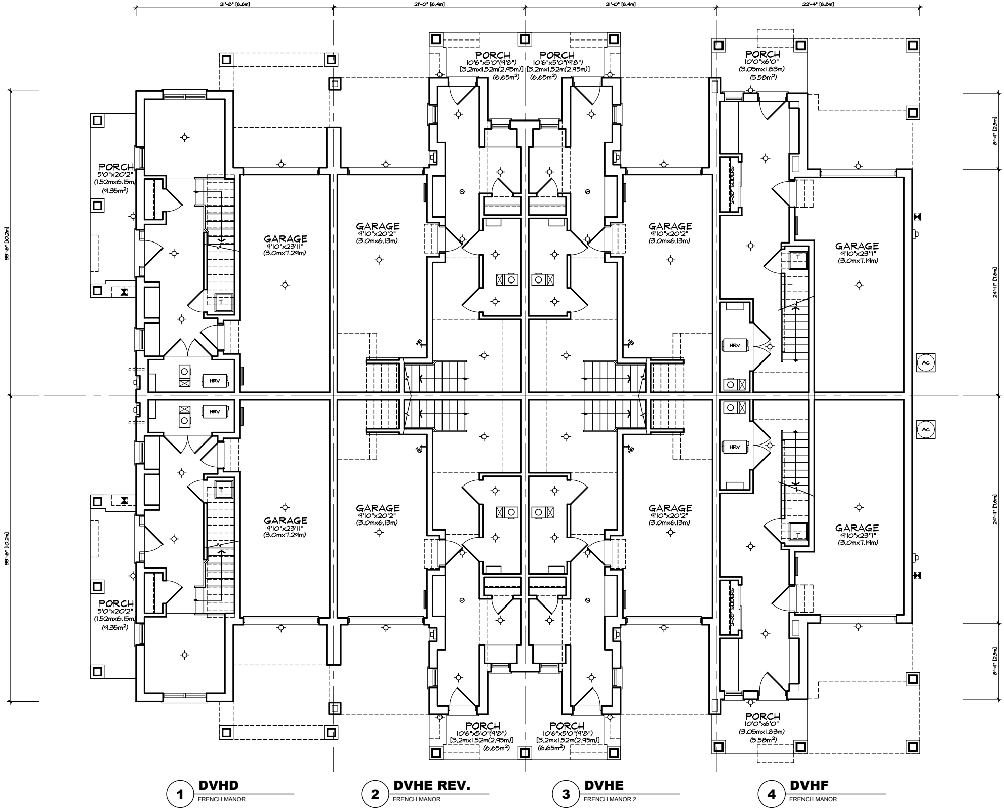
GROUND FLOOR PLAN 'FM' VILLAGE HOMES BLOCK 1
