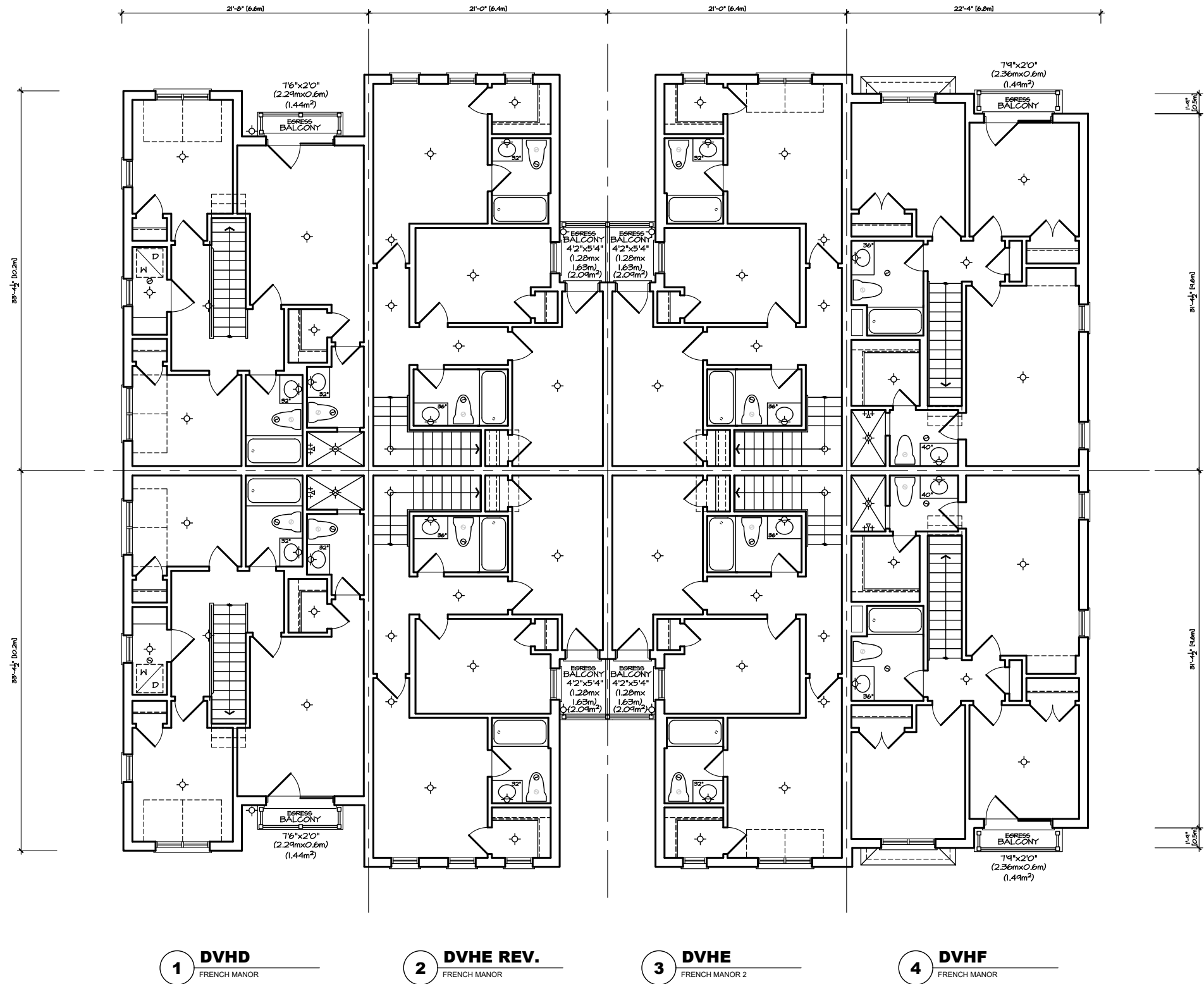
THIRD FLOOR PLAN 'FM' VILLAGE HOMES BLOCK 1
