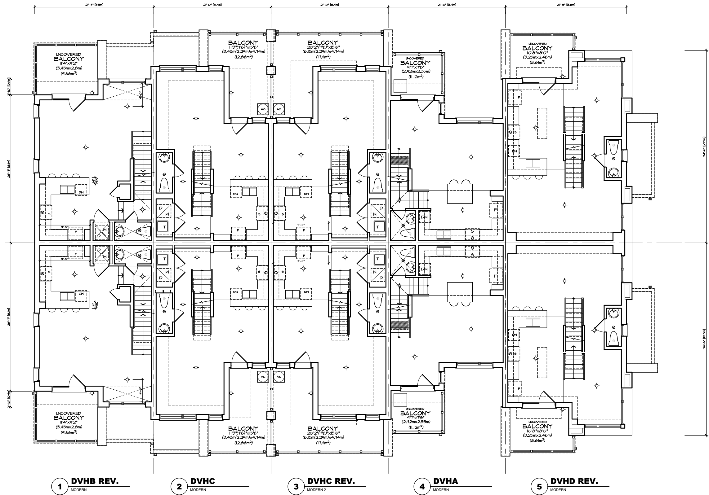
MAIN FLOOR PLAN 'MO' VILLAGE HOMES BLOCK 2
