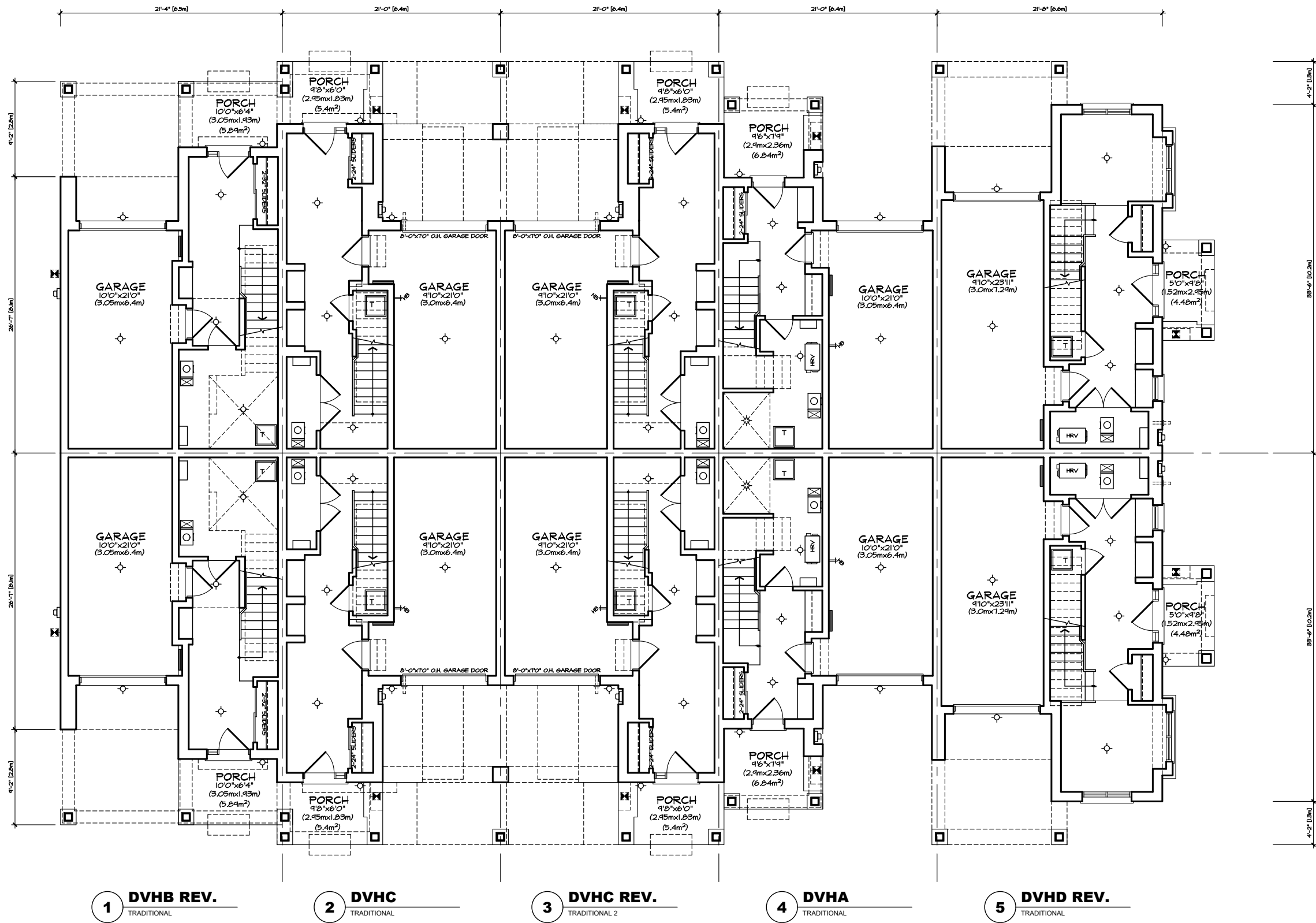
GROUND FLOOR PLAN 'TA' VILLAGE HOMES BLOCK 2
