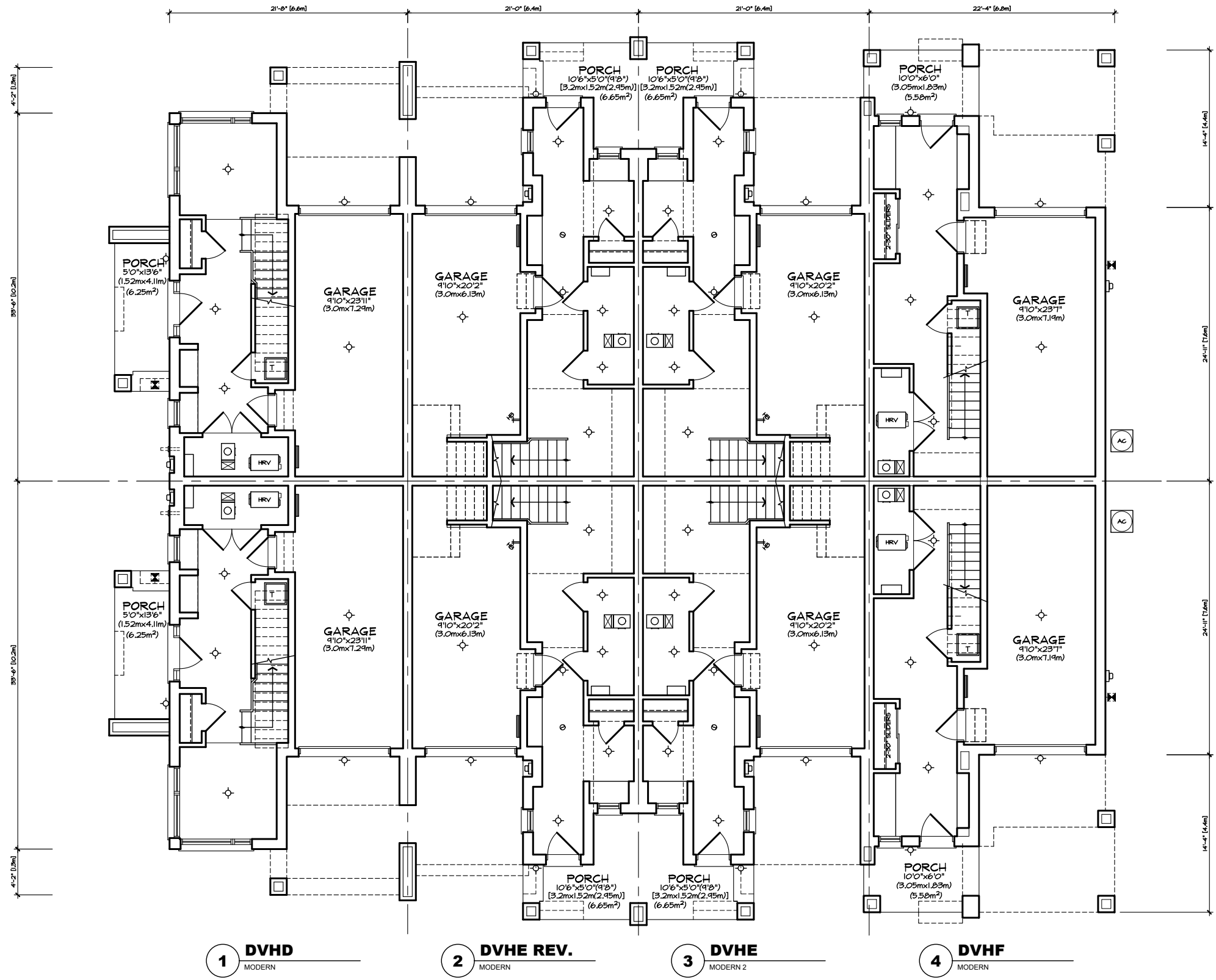
GROUND FLOOR PLAN 'MO' VILLAGE HOMES BLOCK 1
