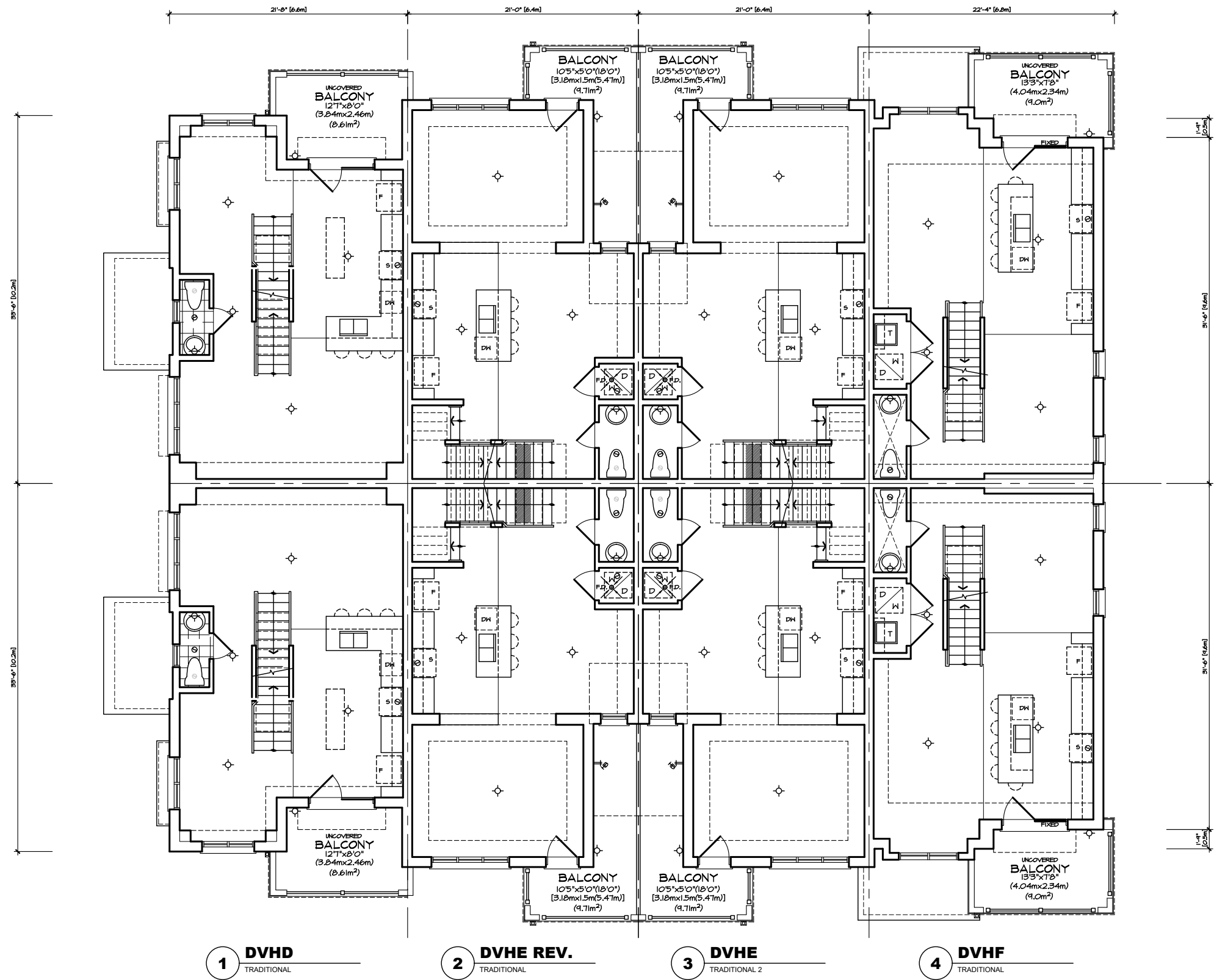
MAIN FLOOR PLAN 'TA' VILLAGE HOMES BLOCK 1
