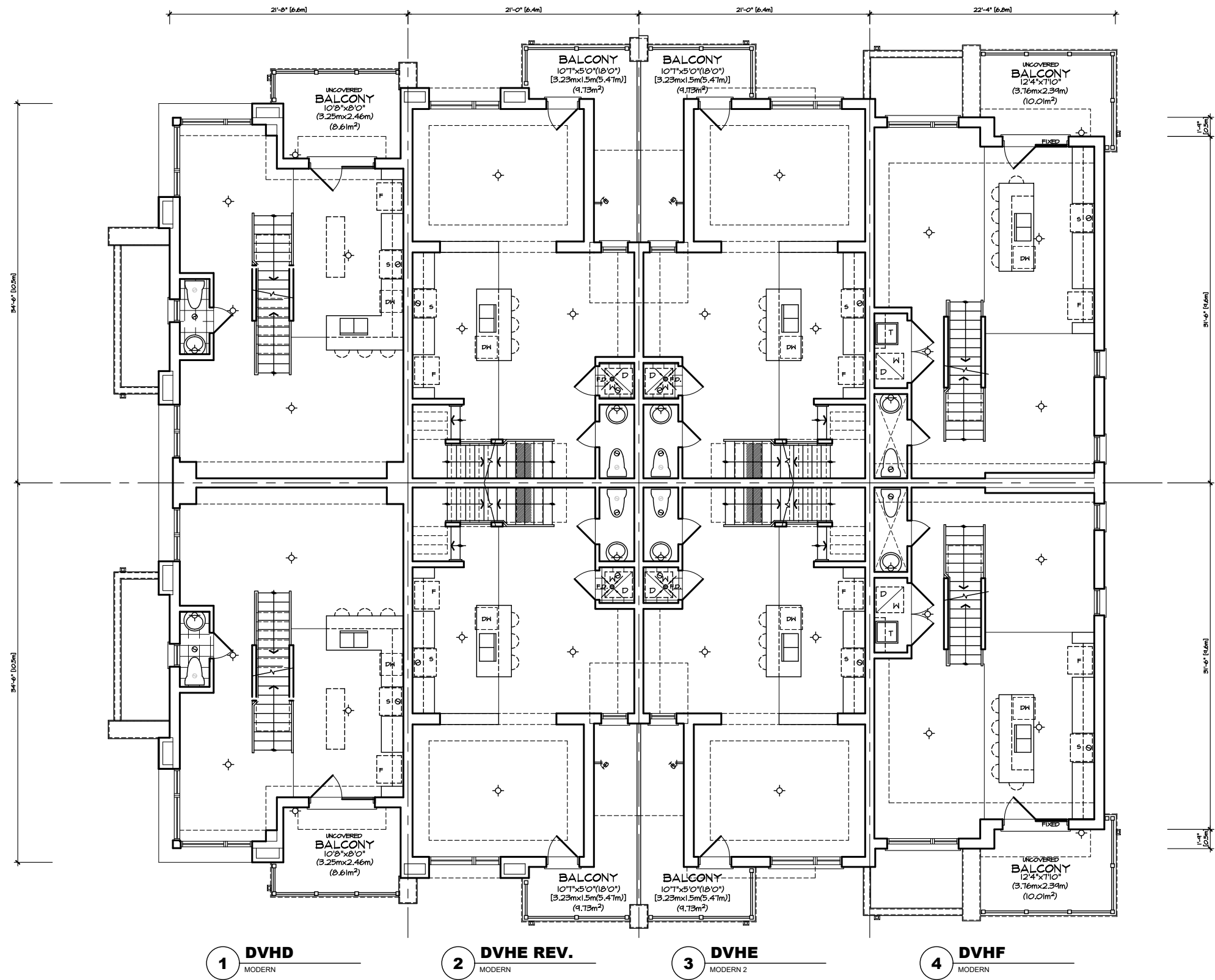
MAIN FLOOR PLAN 'MO' VILLAGE HOMES BLOCK 1
