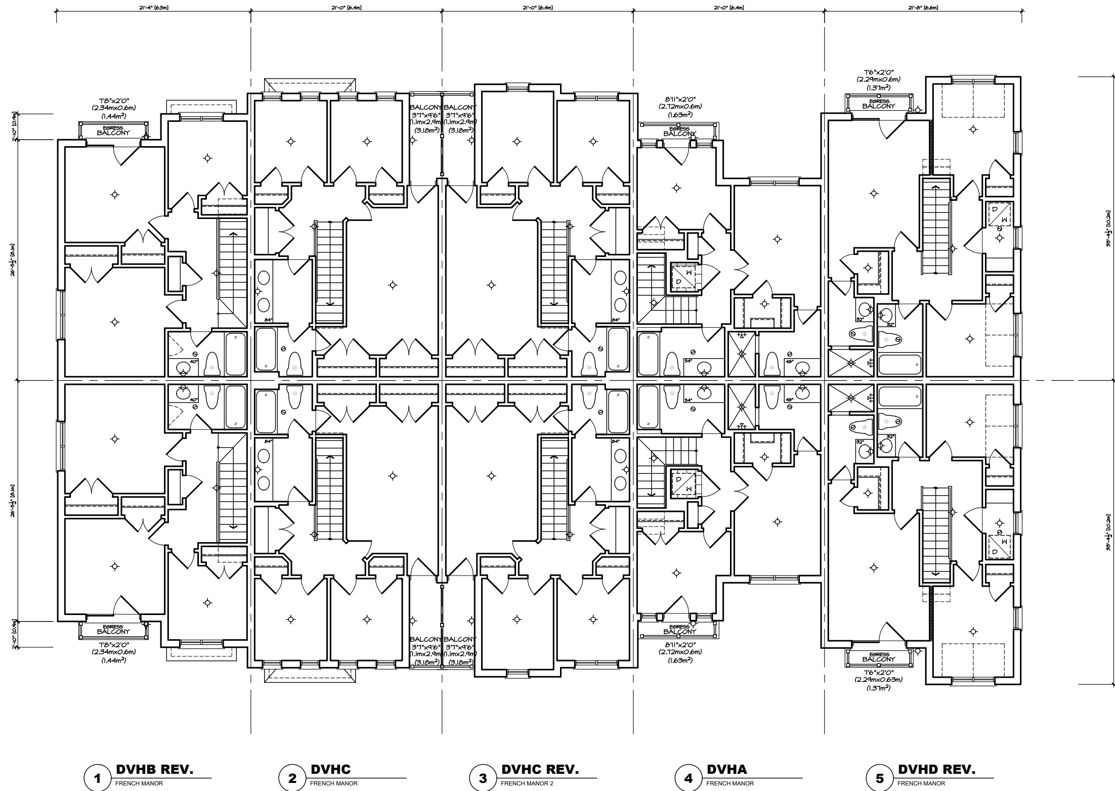
THIRD FLOOR PLAN 'FM' VILLAGE HOMES BLOCK 2
