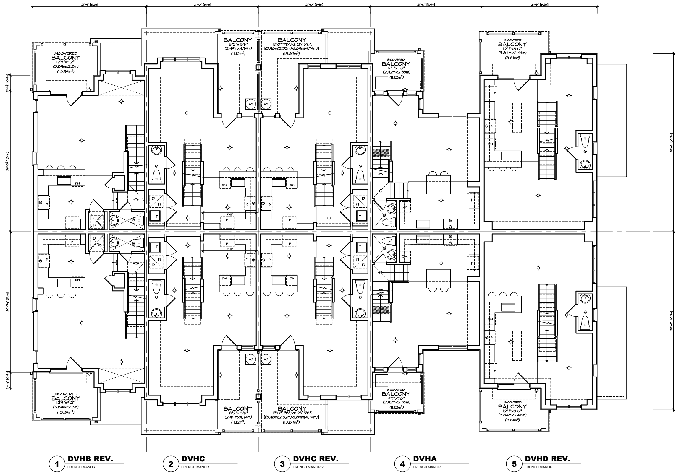
MAIN FLOOR PLAN 'FM' VILLAGE HOMES BLOCK 2
